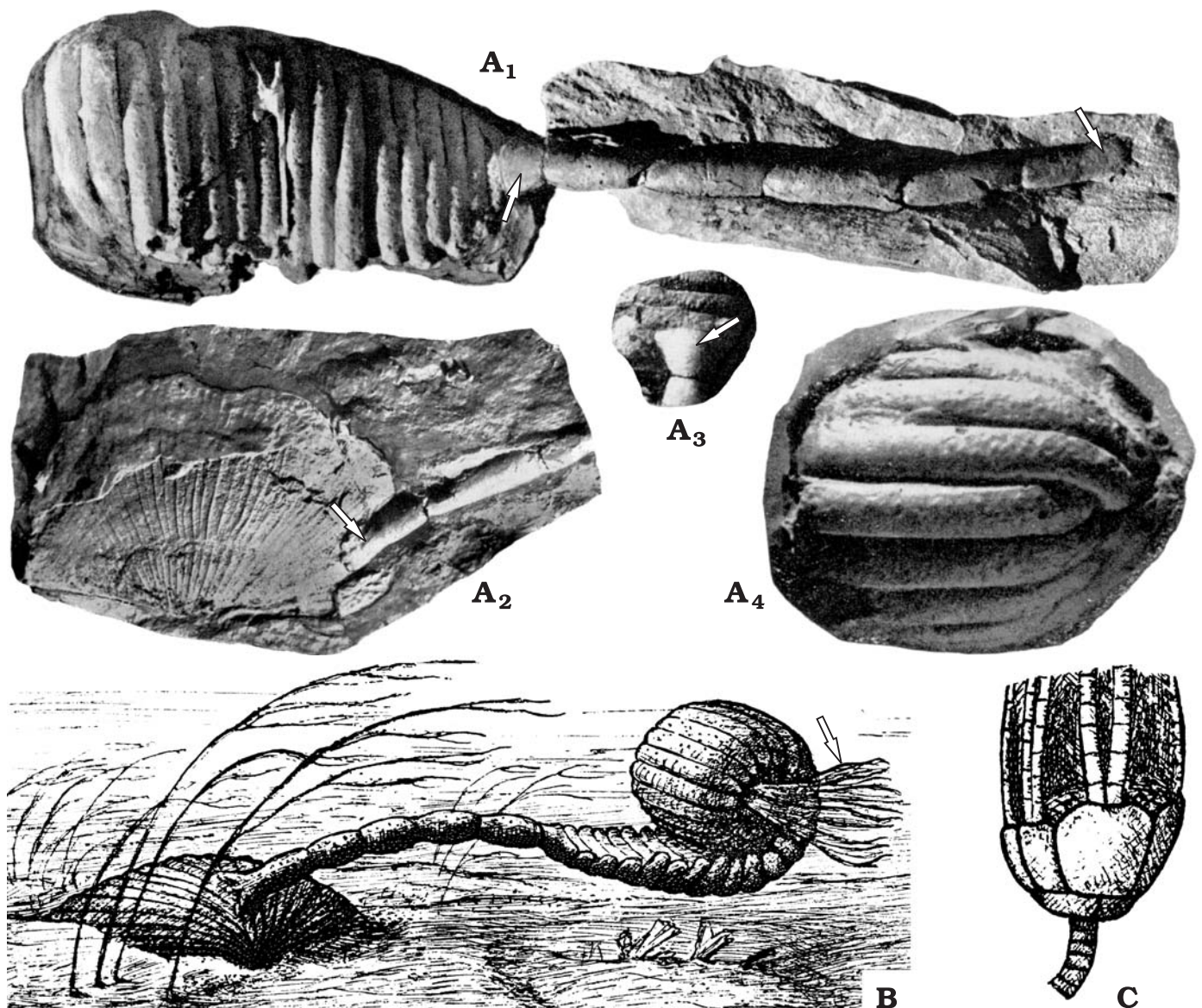
Fig. 3. The lecanocrinid species Ammonicrinus doliiformis Wolburg, 1938a (for 1937) from the Selscheid Formation of Ohle, Sauerland (Wolburg 1938a: 230). A. Casts of nearly complete specimen. Specimen attached to a brachiopod valve (right arrow) ( A_1 ), showing the characteristic triangular connection between mesio- and dististele (left arrow) and slightly compressed mesistele (from Wolburg 1938a: pl. 17: 1); detail view of the attachment disc (arrow) ( A_2 ), encrusting the brachiopod (from Wolburg 1938a: pl. 18: 8); detail view of the triangular connection between mesio- and dististele (arrow) ( A_3 ) (from Wolburg 1938a: pl. 17: 6a); detail view of the coiled, slightly compressed mesistele ( A_4 ) (from Wolburg 1938a: pl. 17: 4). B. Former assumed reconstruction of life mode, figured with a crown that protrudes toward the lateral-exterior (arrow) (from Wolburg 1938a: 240, fig. 5). C. Former assumed reconstruction of the crown (1938a: 233, fig. 4). Not to scale.
