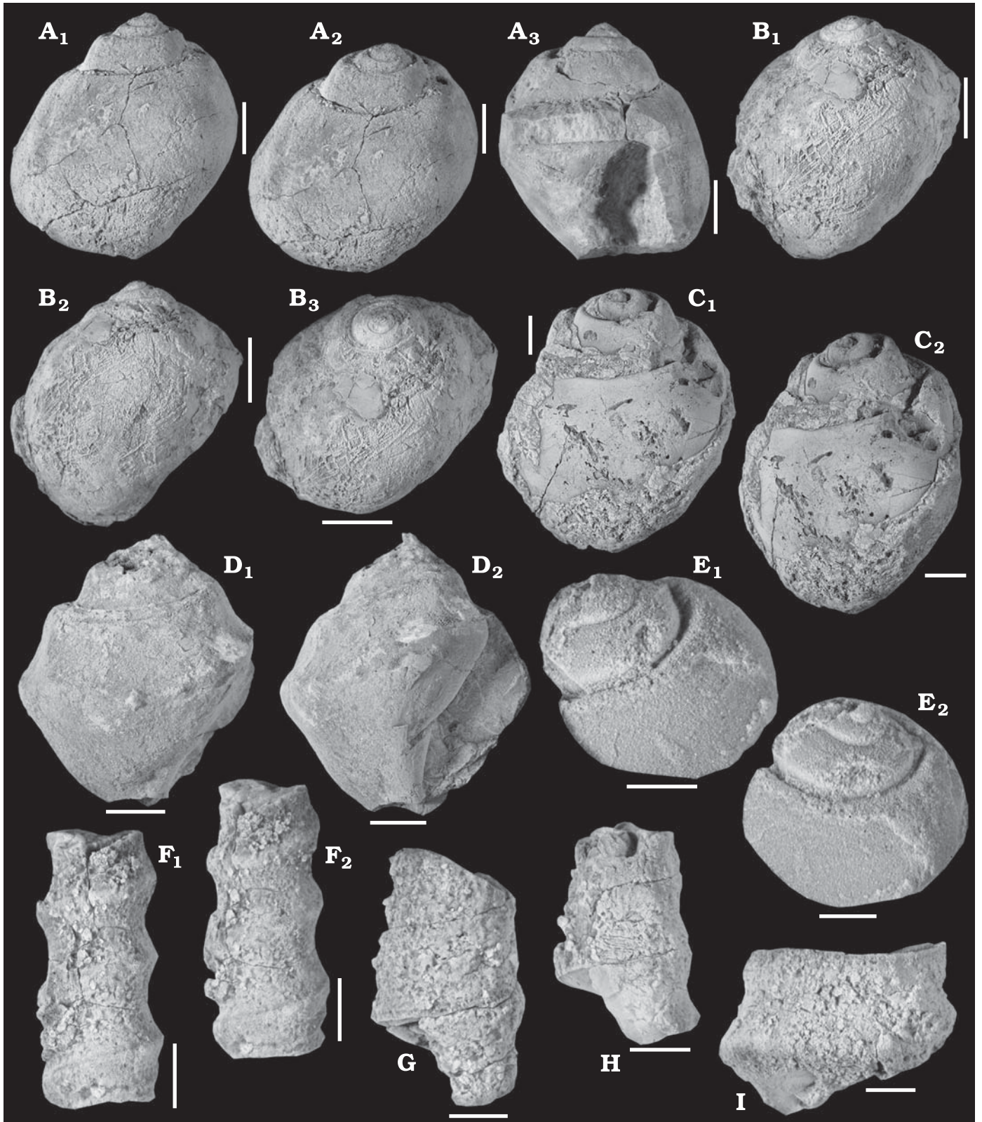
Fig. 4. Early Jurassic gastropods from Lomas Occidentales and Cerro La Trampa fossiliferous localities. A–C. Globularia cf. catanlensis (Weaver, 1931). A. MPEF-PI 4112; teleoconch in lateral (A 1 , A 2 ) and apertural (A 3 ) views. B. MPEF-PI 4114; teleoconch in lateral (B 1 , B 2 ) and latero-apical (B 3 ) views. C. MPEF-PI 4116, teleoconch in lateral views (C 1 , C 2 ). D. Globularia sp. MPEF-PI 4119; teleoconch in lateral (D 1 ) and apertural (D 2 ) views. E. Naricopsina? sp.; MPEF-PI 3560, teleoconch in latero-apical views (E 1 , E 2 ). F. Nerinea? sp. 1. MPEF-PI 4123, fragmentary teleoconch in lateral views (F 1 , F 2 ). G–I. Nerinea? sp. 2. G. MPEF-PI 4124, fragmentary teleoconch in lateral view. H. MPEF-PI 4125, fragmentary teleoconch in lateral view. I. MPEF-PI 4126, fragment of last teleoconch whorl in lateral view. Scale bars: A–D 10 mm, E–I 3 mm.
