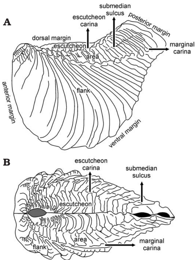
Fig. 1. Schematic drawing of the shell of an adult specimen of Myophorella garatei Leanza, 1981 showing the main features of trionioides shell morphology. A. Left lateral view. B. Dorsal view.
