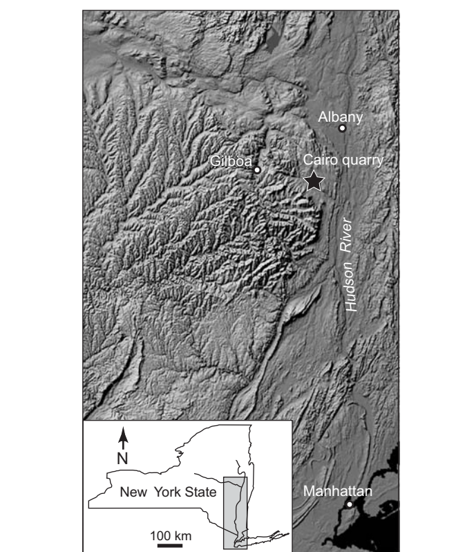
Fig. 1. Location of the Cairo quarry (star) (3.22 km northwest of Cairo, Greene County, 42.32° N and 74.04° W, NAD 83) in eastern New York State, USA (inset map); figure modified from Hernick et al. (2008: fig. 1).
