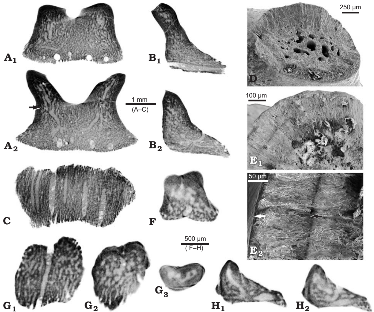
Fig. 6. Internal structure of the teeth of omalodontid shark Portalodus mannoliniae sp. nov. from the Givetian of the Cairo quarry, New York, for the adult (A–E) and the juvenile (F–H) morphotypes. A–C. NYSM 17718; images acquired by micro CT-scan (exposure time: 1300 ms; accelerating voltage: 75kV; current: 106 \mu A). A. Coronal planes angled through the crown and the base, near the lingual margin, with the base horizontal (A 1 ) and along the plane of the cusps (A 2 ), black arrow indicates a possible growth line in the orthodontine outer layer. B. Transverse planes through the right (B 1 ) and the left (B 2 ) cusps when looking from the labial side. C. Horizontal plane through the base. D–E. NYSM 17716; images acquired by SEM. D. Break facet of the right cusp when looking from the labial side. E. Close-up view of the margin of the left cusp (when looking from the labial side) (E 1 ) and of the orthodontine external layer (E 2 ); white arrow indicates the enamel outer layer, black arrow shows separation line between the two main orthodontine layers. F–H. NYSM 17699; images acquired by micro CT-scan (exposure time: 1000 ms; accelerating voltage: 70kV; current: 114 \mu A). F. Coronal plane angled through the crown and the base. G. Horizontal planes through the base, near the bottom of the base (G 1 ), at about mid-base (G 2 ), and at the bottom of the crown, underneath the forking of the cusps (G 3 ). H. Planes along the labio-lingual axis through the left cusp (when looking from the labial side), near its median side (H 1 ), and inbetween the two cusps (H 2 ).
