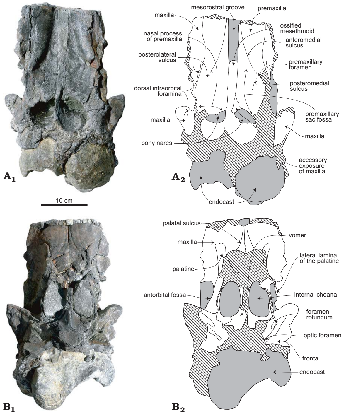
Fig. 2. Cranium of Globicephalinae gen. et sp. indet. 1 (UCMP 219223, Seacliff Beach skull), Pliocene, UCMP locality V99879, in dorsal ( A ) and ventral ( B ) views. Cross-hatching denotes damaged or missing bone, gray indicates matrix (including the endocast). Photographs ( A 1 , B 1 ), interpretative line drawings ( A 2 , B 2 ).
