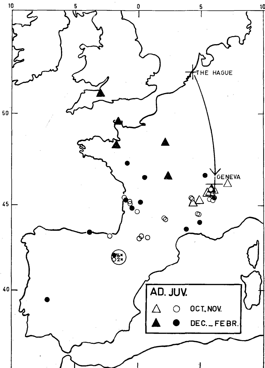
Fig. 7. Recoveries of Starlings in the same season, after displacement to Geneva.
