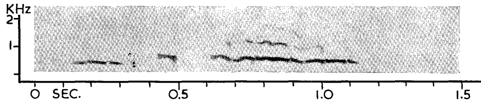
Spectrograms of the most common calls of male Black Grouse.
