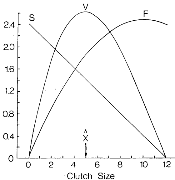
Fig. 3. Model of optimal clutch size. Fitness ( V ) equals the product of longevity ( S , number of breeding seasons) and fecundity ( F , expected number of offspring surviving from a given breeding season). The optimal clutch size ( \bar{x} ) maximizes V .
