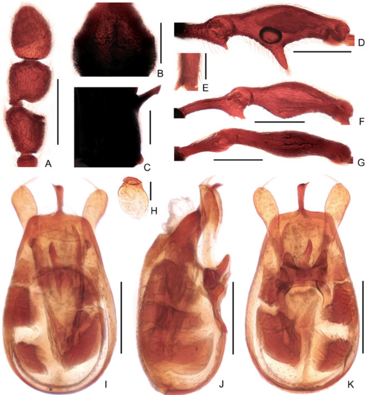
Fig 9. Male diagnostic features of Pselaphodes khandbarius sp. nov. (A) Antennal club. (B) Pronotum. (C) Metaventral process, in lateral view. (D) Protrochanter and profemur. (E) Apex of protibia. (F) Mesotrochanter and mesofemur. (G) Metatrochanter and metafemur. (H) Sternite IX. (I-K) Aedeagus, in dorsal (I), lateral (J), and ventral (K) view. Scale bars: 0.3 mm in A-B, D, F-G; 0.2 mm in C, I-K; 0.1 mm in E, H.
