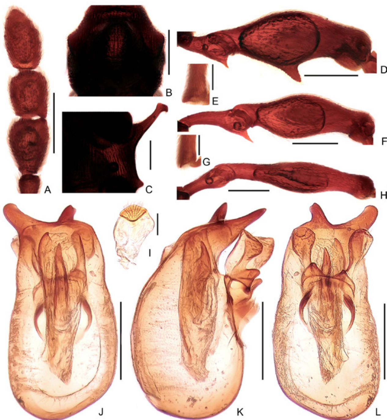
Fig 5. Male diagnostic features of Pselaphodes bilobatus sp. nov. (A) Antennal club. (B) Pronotum. (C) Metaventral process, in lateral view. (D) Protrochanter and profemur. (E) Apex of protibia. (F) Mesotrochanter and mesofemur. (G) Apex of mesotibia. (H) Metatrochanter and metafemur. (I) Sternite IX. (J-L) Aedeagus, in dorsal (J), lateral (K), and ventral (L) view. Scale bars: 0.3 mm in A-B, D, F, H; 0.2 mm in C, J-L; 0.1 mm in E, G, I.
