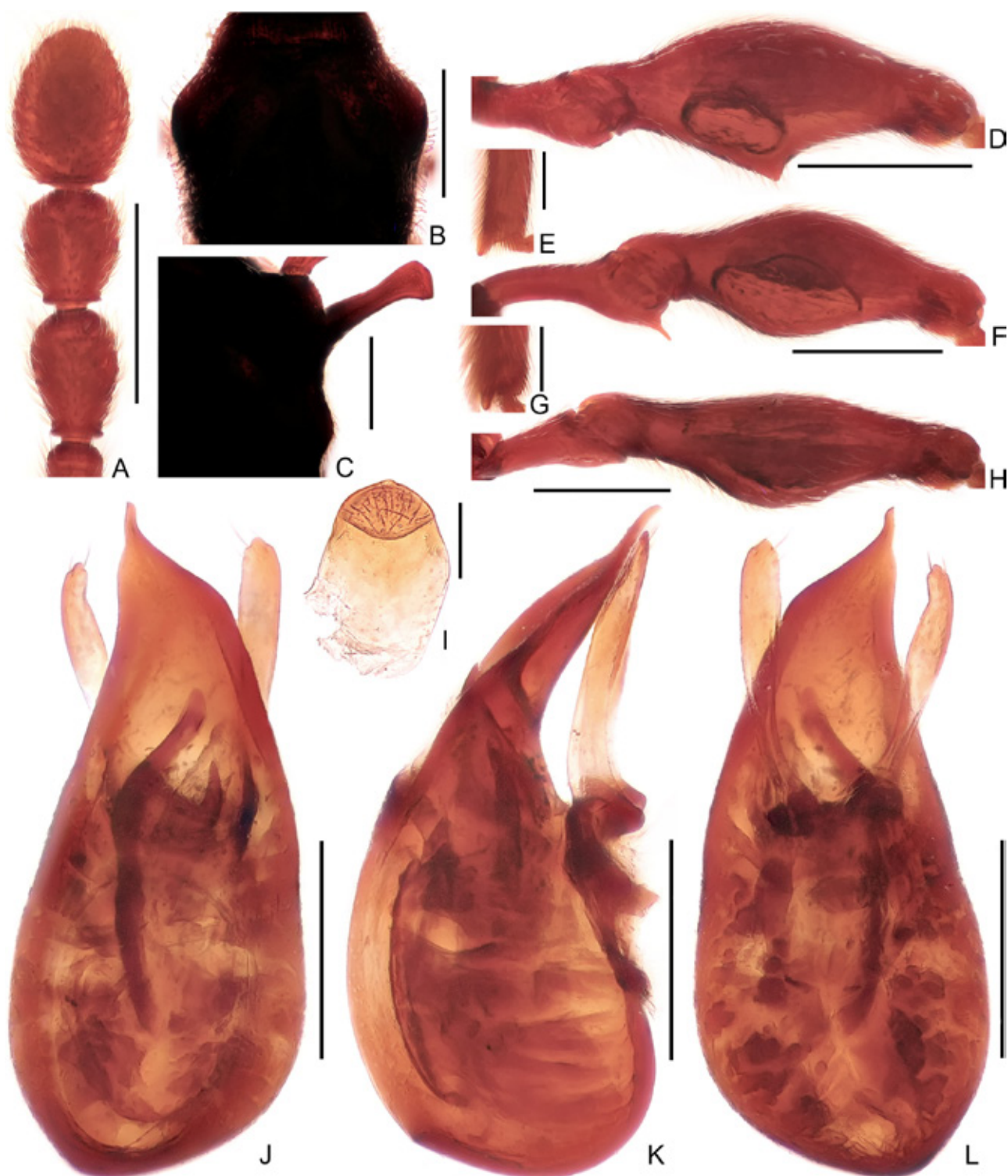
Fig 2. Male diagnostic features of Pselaphodes ampliatus sp. nov. (A) Antennal club. (B) Pronotum. (C) Metaventral process, in lateral view. (D) Protochanter and profemur. (E) Apex of protibia. (F) Mesotrochanter and mesofemur. (G) Apex of mesotibia. (H) Metatrochanter and metafemur. (I) Sternite IX. (J-L) Aedeagus, in dorsal (J), lateral (K), and ventral (L) view. Scale bars: 0.3 mm in A-B, D, F, H; 0.2 mm in C, J-L; 0.1 mm in E, G, I.
