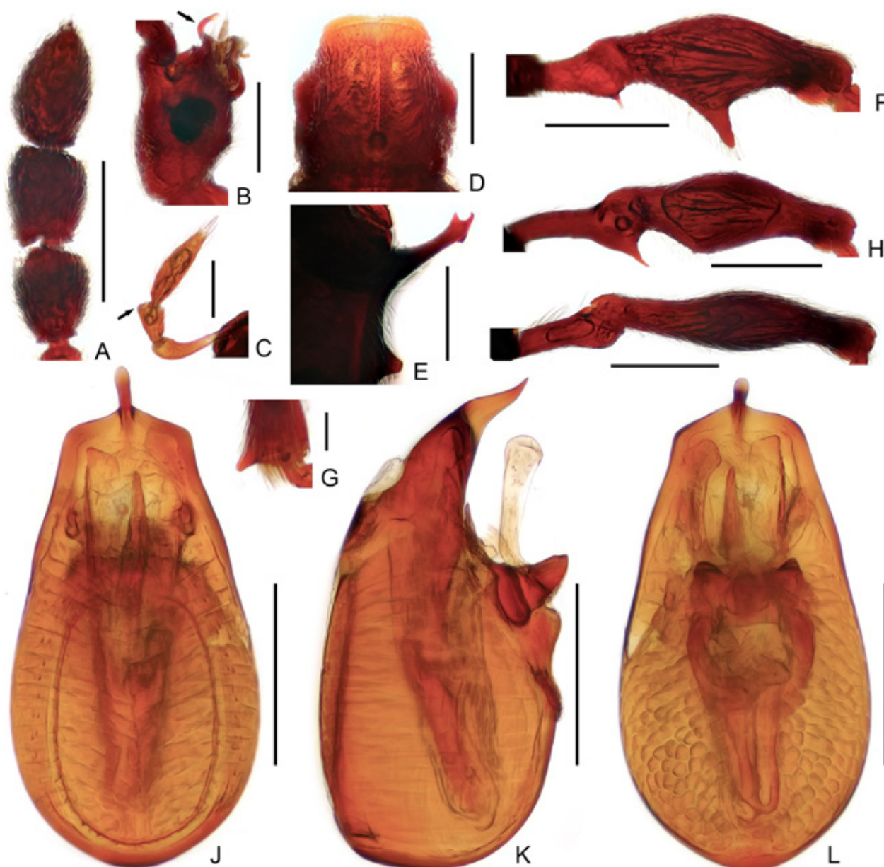
Fig 24. Male diagnostic features of Pselaphodes unicornis . (A) Antennal club. (B) Head, in lateral view. (C) maxillary palpus. (D) Pronotum. (E) Metaventral process. (F) Protrochanter and profemur. (G) Apex of protibia. (H) Mesotrochanter and mesofemur. (I) Metatrochanter and metafemur. (J-L) Aedeagus, in dorsal (J), lateral (K), and ventral (L) view. Scale bars: 0.3 mm in A, B, D, F, H, I; 0.2 mm in E, J-L; 0.1 mm in C; 0.05 mm in G.
