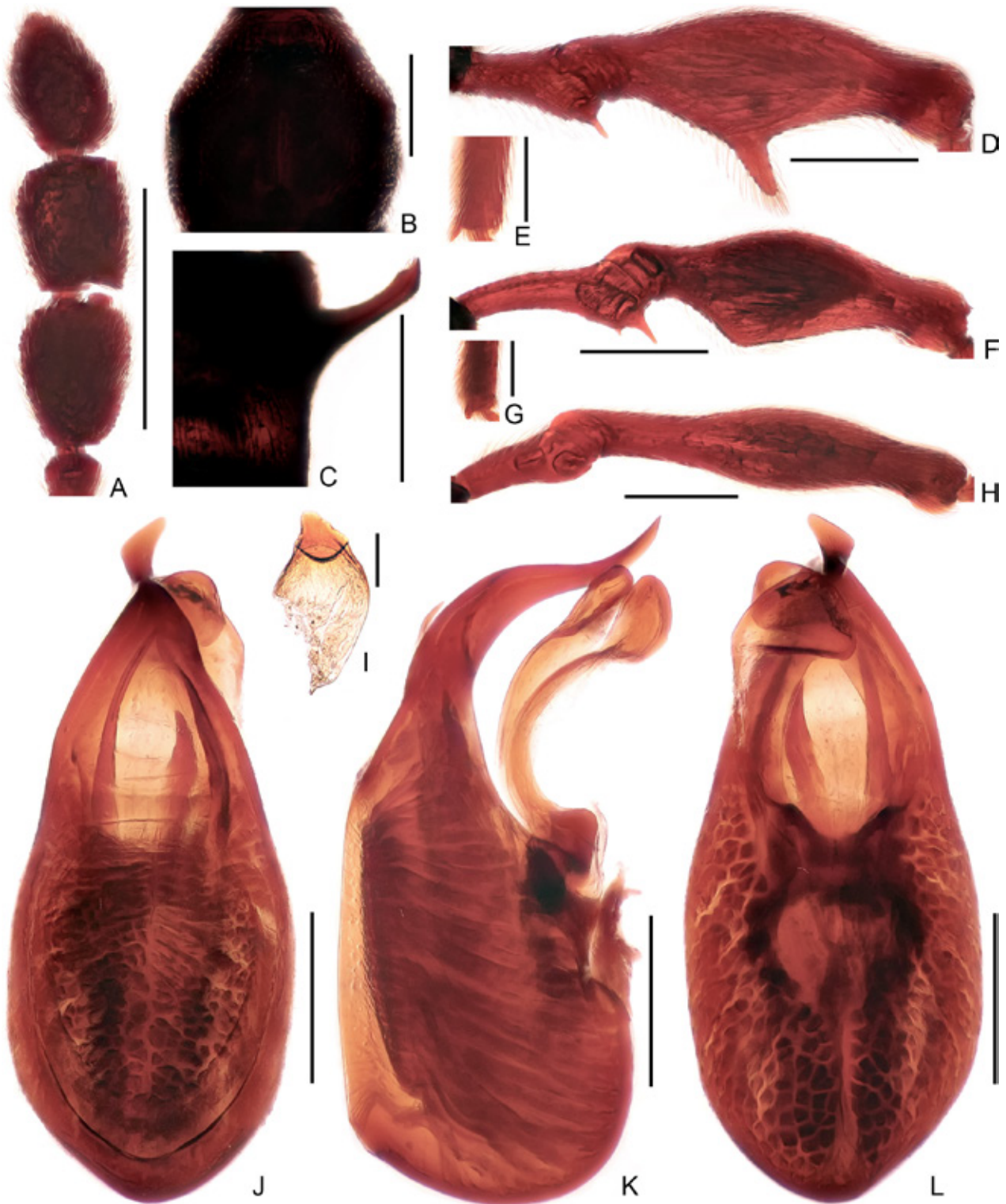
Fig 14. Male diagnostic features of Pselaphodes psomus sp. nov. (A) Antennal club. (B) Pronotum. (C) Metaventral process, in lateral view. (D) Protrochanter and profemur. (E) Apex of protibia. (F) Mesotrochanter and mesofemur. (G) Apex of mesotibia. (H) Metatrochanter and metafemur. (I) Sternite IX. (J-L) Aedeagus, in dorsal (J), lateral (K), and ventral (L) view. Scale bars: 0.3 mm in A-B, D, F, H; 0.2 mm in C, J-L; 0.1 mm in E, G, I.
