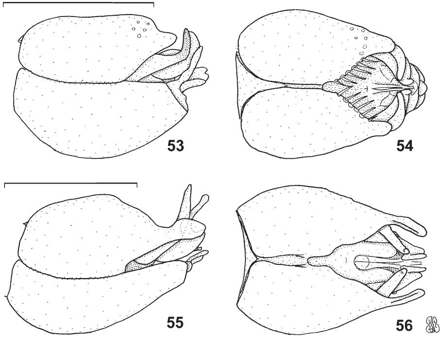
Figs 53–56. Trichardis species, male genitalia: (53, 54) lateral and ventral of T. zinidi sp. n., holotype; (55, 56) lateral and ventral of T. indica sp. n., holotype. Scale lines = 1 mm.
