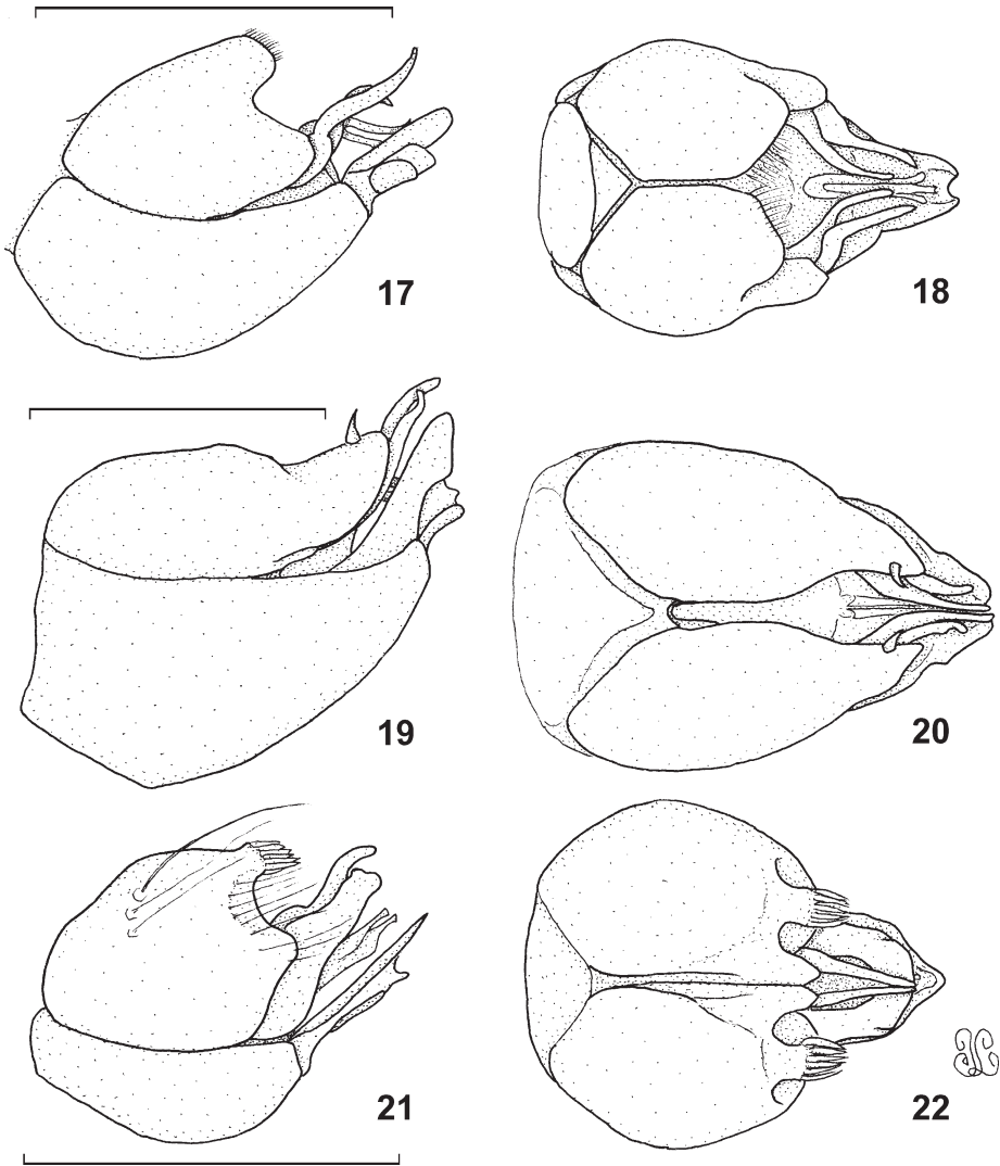
Figs 17–22. Trichardis species, male genitalia: (17, 18) lateral and ventral of T. glabra sp. n., paratype, Bansang; (19, 20) lateral and ventral of T. grisescens Engel, 1924, holotype; (21, 22) lateral and ventral of T. hesperia sp. n., paratype, Kayes. Scale lines = 1 mm.
