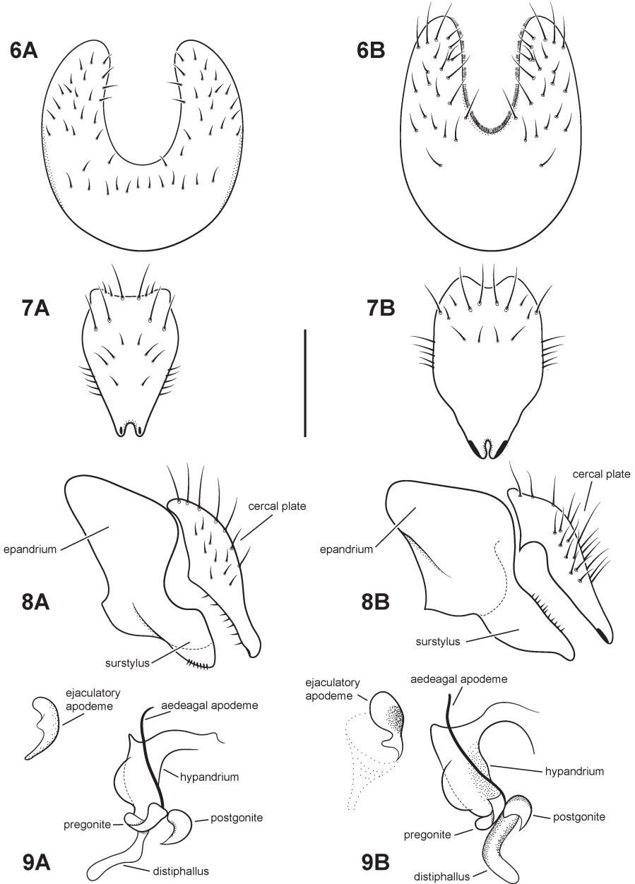
Figs 6–9. Coenosia macrotriseta sp. n., ♂ (A) and C. globuliseteta Pont, ♂ (B): (6) sternite 5, dorsal view; (7) cercal plate, dorsal view; (8) epandrium, surstylus and cercal plate, lateral view; (9) phallic complex, lateral view. Scale bar = 0.2 mm.
