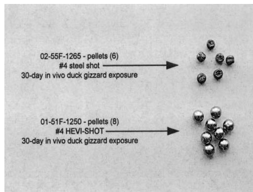
FIGURE 1. Photograph showing the physical condition of No. 4 steel shot and No. 4 H-S after 30 days in mallard gizzards when mallards were fed 100% whole kernal corn diet with quartzite grit available ad libitum . This photo is representative of the final condition of the two types of shot across all ducks examined.
