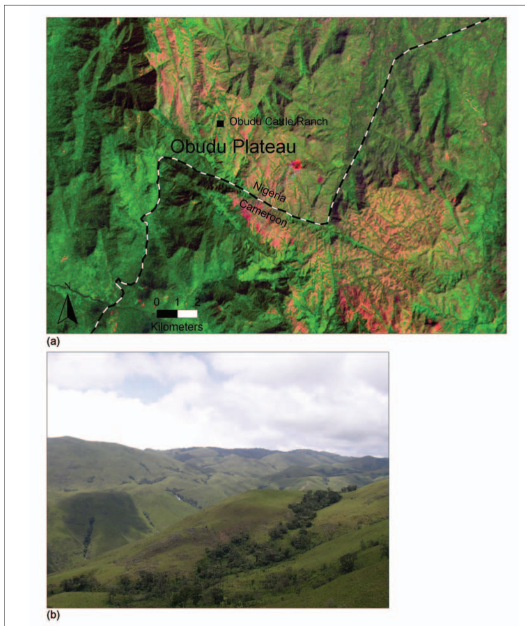
Figure 21. (a) Satellite image (Landsat 7; December 2000) of the highland area along the Nigerian-Cameroon border showing the dissected nature of the area. Pink areas are probably recently burned grassland and human settlements (for instance, the Balegete villages in the southwestern corner of this scene). (b) A view of the Obudu Plateau looking WNW from near the Obudu Cattle Ranch, September 2002.
