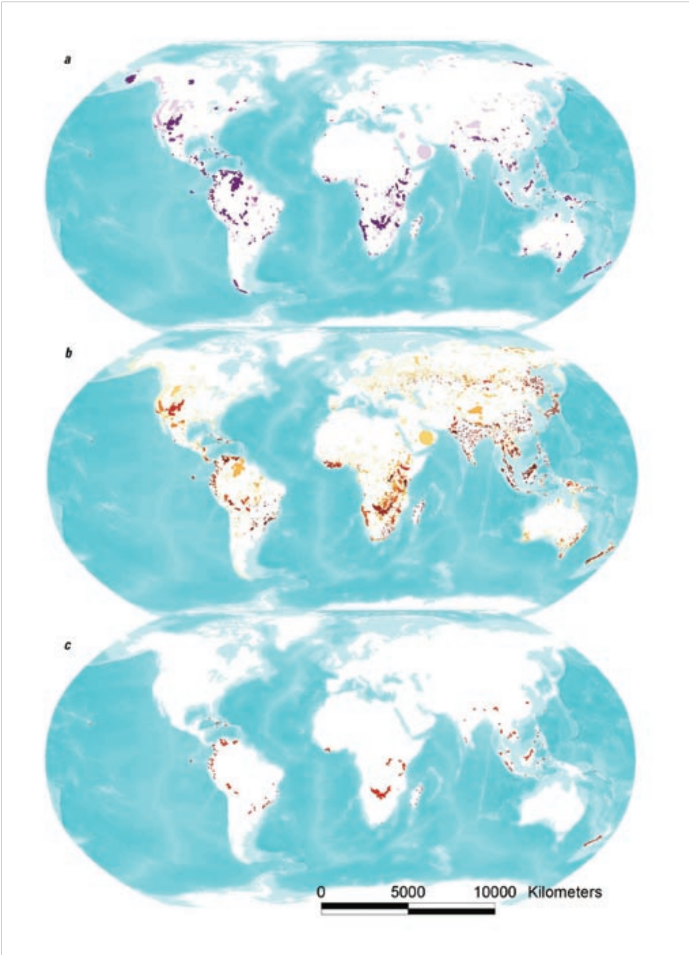
Figure 4.5 Global distribution of (a) irreplaceability, (b) threat, and (c) urgency for the conservation of threatened birds among protected sites, as obtained in Scenario B. Darker shades in (a) and (b) correspond to higher values of irreplaceability and threat.
