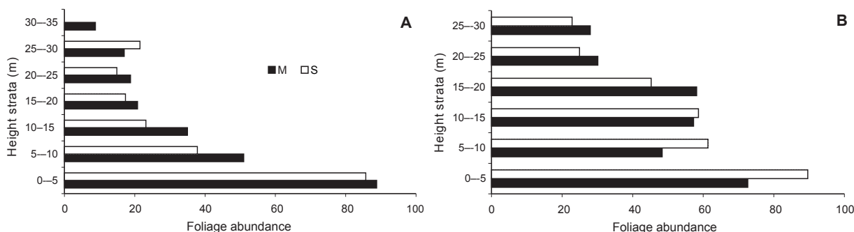
Fig. 2 Foliage height profile: A, in evergreen forest (EV) B, in moist deciduous forest (MD) in monsoon season (M) and summer (S).
