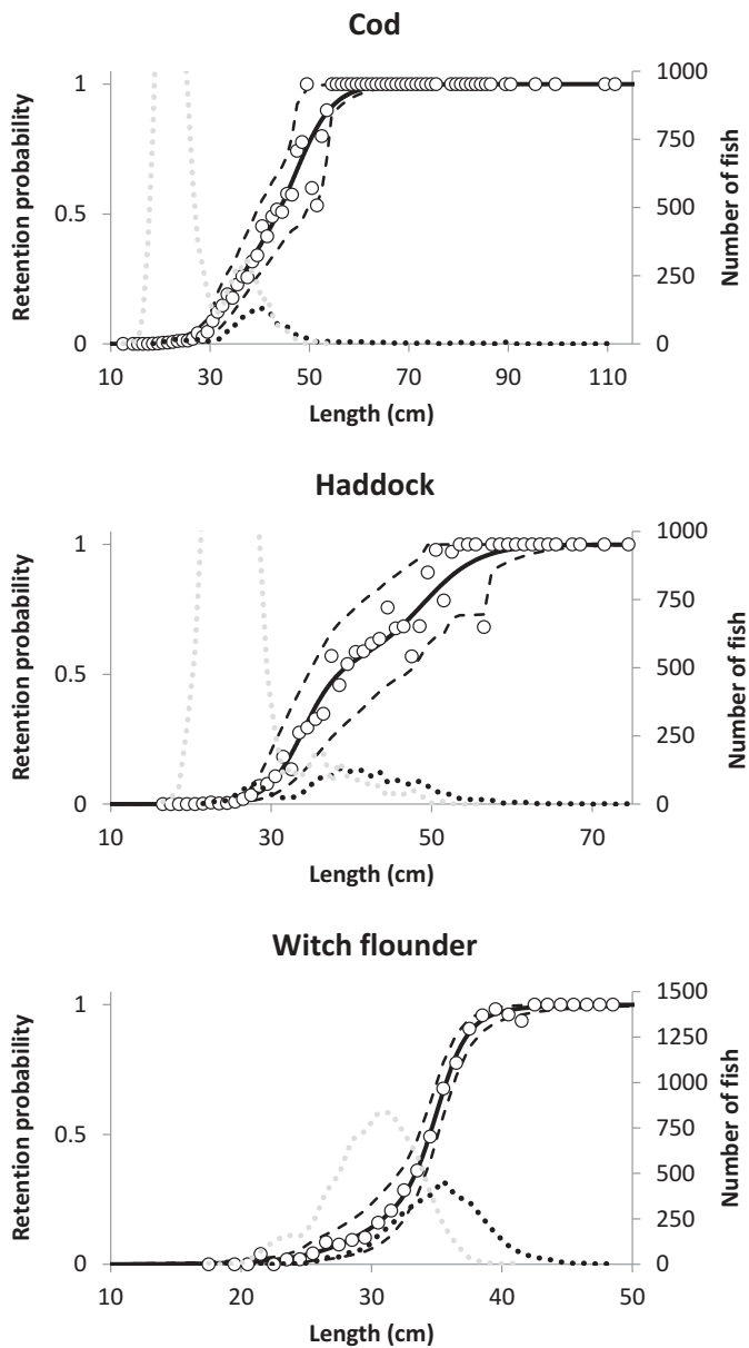
FIGURE 3. Size selection curves (probability of retention in the cod end or cover as a function of fish length) for three species. Circles represent the experimental retention rates; black lines represent the modelled size selections; dashed lines represent the 95% confidence limits for the estimated size selection curves; black dotted lines represent the population retained in the cod end; and gray dotted lines represent the populations collected in the cod end cover.
