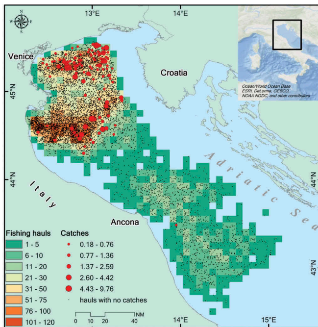
FIGURE 1. Map of the study area in the north-central Adriatic Sea, showing the spatial distribution of fishing effort and catches (CPUE, number of individuals per 10^6 \text{ m}^3 ) of (a) Common Eagle Rays and (b) Bull Rays during 2006–2012.
