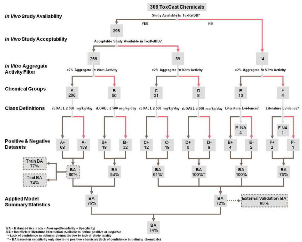
FIG. 1. Decision tree diagram representing the process by which the 309 ToxCast chemicals were grouped, based on in vivo study acceptability/availability and in vitro aggregate bioactivity, and subsequently defined as positive or negative for reproductive toxicity, based on having achieved an rLOAEL of less than 500 mg kg -1 day -1 . Applying the model developed using chemical group A to all other chemical groups, individual and combined balanced accuracy values (average of sensitivity and specificity) summarize the results across the entire chemical library and provide context and summary information; each chemical group is discussed in greater detail throughout the Results and Discussion sections.
