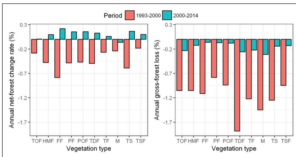
Figure 3. Annual net-forest change and gross forest loss rates (%) in the natural vegetation types. TOF = tropical oak forest; HMF = humid montane forest; FF = fir forest; PF = pine forest; POF = pine-oak forest; TDF = tropical deciduous forest; TF = tropical forest; M = mangrove; TS = tropical scrub; TSF = tropical semideciduous forest in Central Veracruz, Mexico, for the periods 1993 to 2000 and 2000 to 2013.
