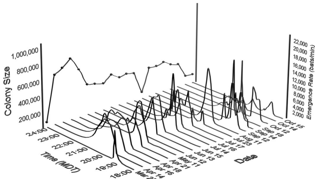
FIG. 1. —Seasonal and nightly changes in colony size, onset, duration, and rate of emergence of Brazilian free-tailed bats ( Tadarida brasiliensis ) at Carlsbad Cavern, New Mexico, based on 20 censuses in 2005 (seasonal axis not to scale).
