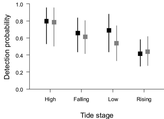
FIGURE 3. Estimated probability of detecting American Oystercatcher pairs (black) or individuals (gray) as a function of tide stage. Values are presented for the average survey date (May 24).
