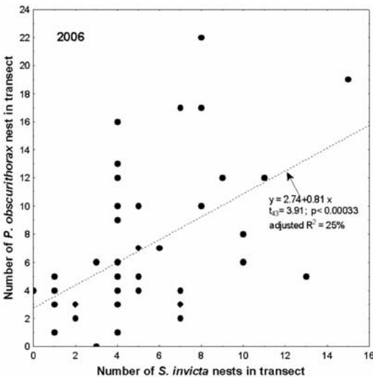
Fig. 6. The densities of fire ant nests in relationship to the densities of P. obscurithorax nests in the 2006 survey.
