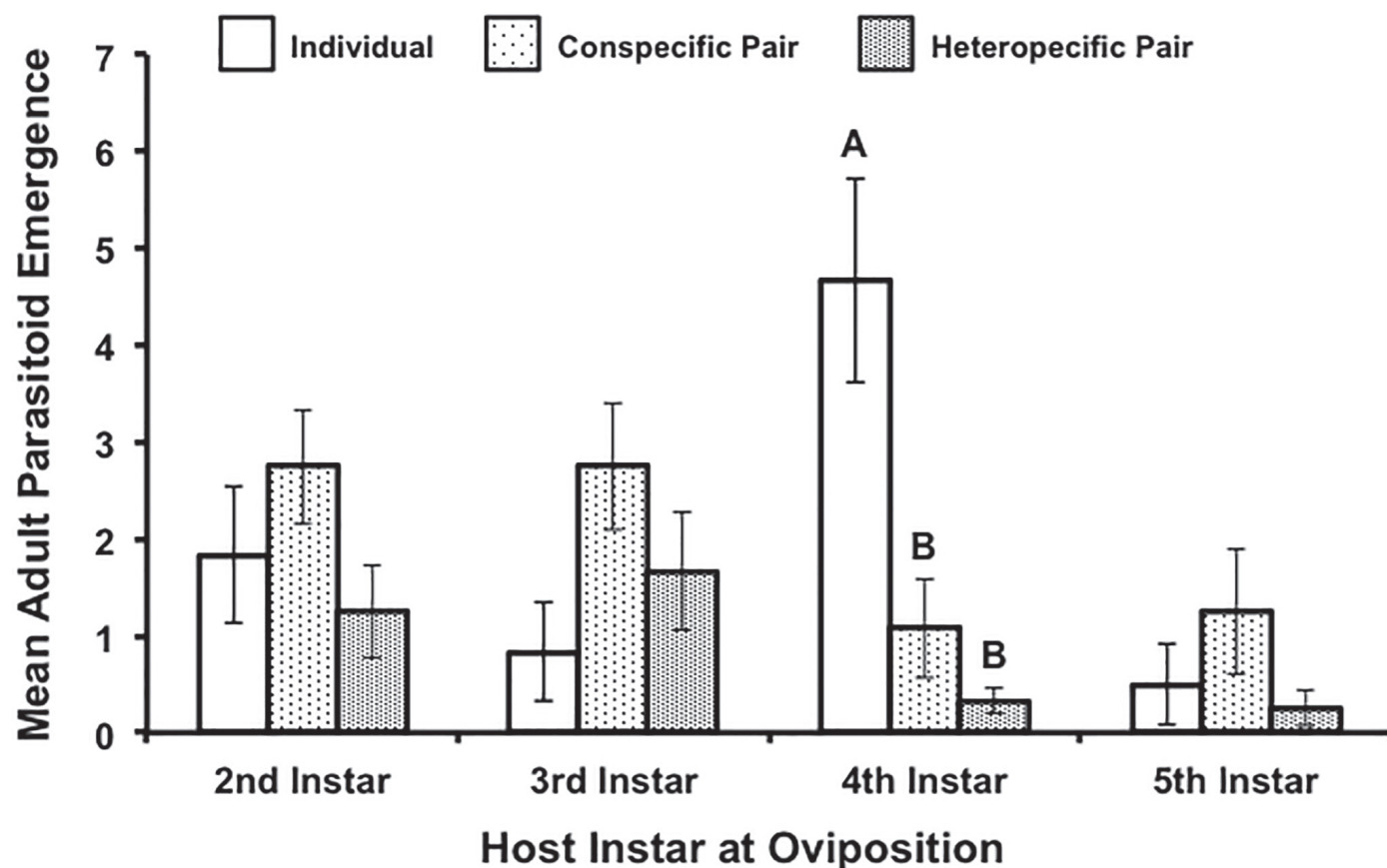
Fig. 3. Mean ( \pm SE) emergence of adult Diaphorencyrtus aligarhensis from second through fifth instar Diaphorina citri nymphs in no-choice experiments when females foraged alone or with hetero- and conspecific competitors. Foraging scenario only affected parasitoid emergence when D. aligarhensis foraged for fourth instar D. citri nymphs (means with the same letters are not significantly different; P > 0.05 ).
