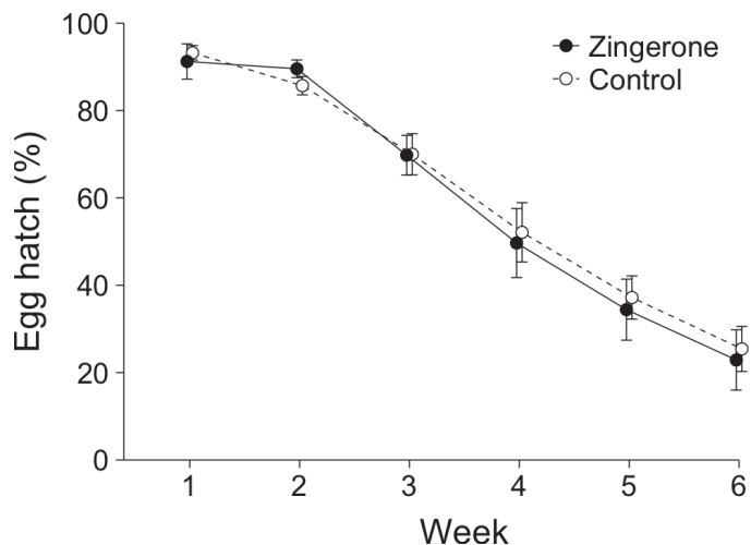
Fig. 3. Percent hatch rate (mean \pm SE) of eggs laid by females mated to zingerone-fed and unfed (control) males. Fifty eggs were observed 3 times each wk and the hatch rate was averaged weekly. Means represent the weekly hatch rate of eggs collected from 6 cages containing 15 mated females each.
