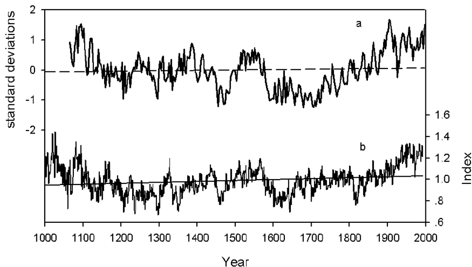
FIGURE 7. Comparison of (a) temperature variations (standard deviations) around mean obtained from tree-ring width and carbon stable isotope in tree-rings in middle Qilian Mountains, and (b) temperature proxy “North Hemispheric regional curve standardization chronology” from Esper et al. (2002). The dashed lines show the trends over the entire periods of the series.
