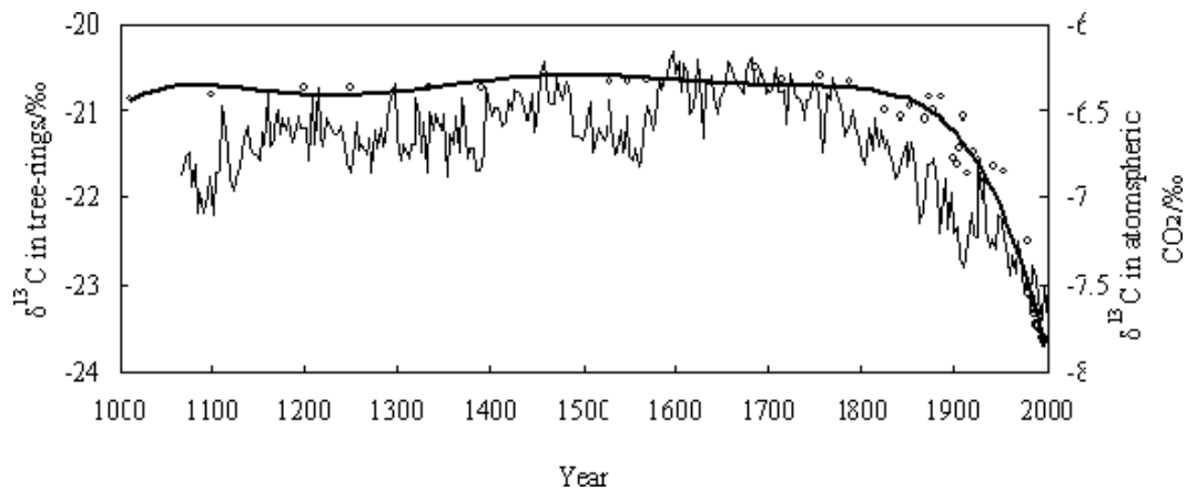
FIGURE 3. Raw averaged 3-yr groups \delta^{13}\text{C} -records of tree-ring cellulose from Qilian juniper and \delta^{13}\text{C} in atmospheric \text{CO}_2 covering the period from 1060 to 2000. Open points show the \delta^{13}\text{C} data in atmospheric \text{CO}_2 from ice-core (Francey et al., 1999; Trudinger et al., 1999).
