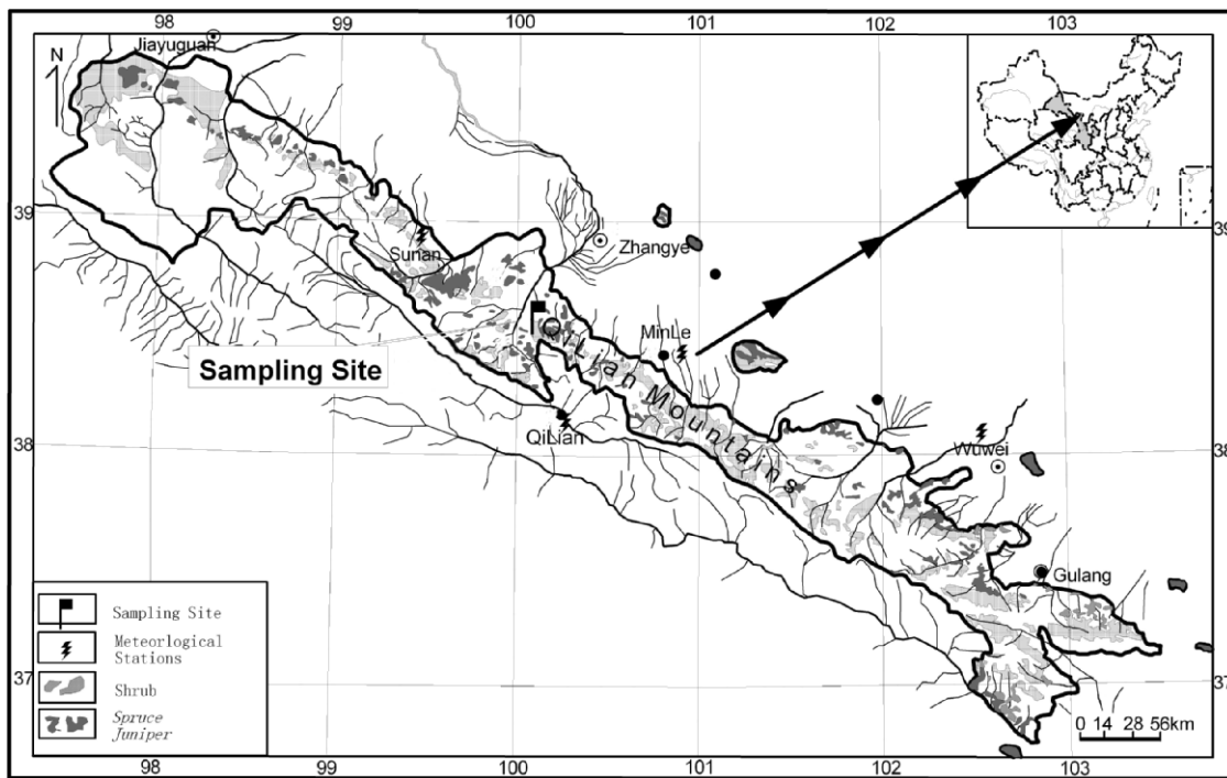
FIGURE 1. Location of tree-ring sampling site and meteorological stations used in this study.
