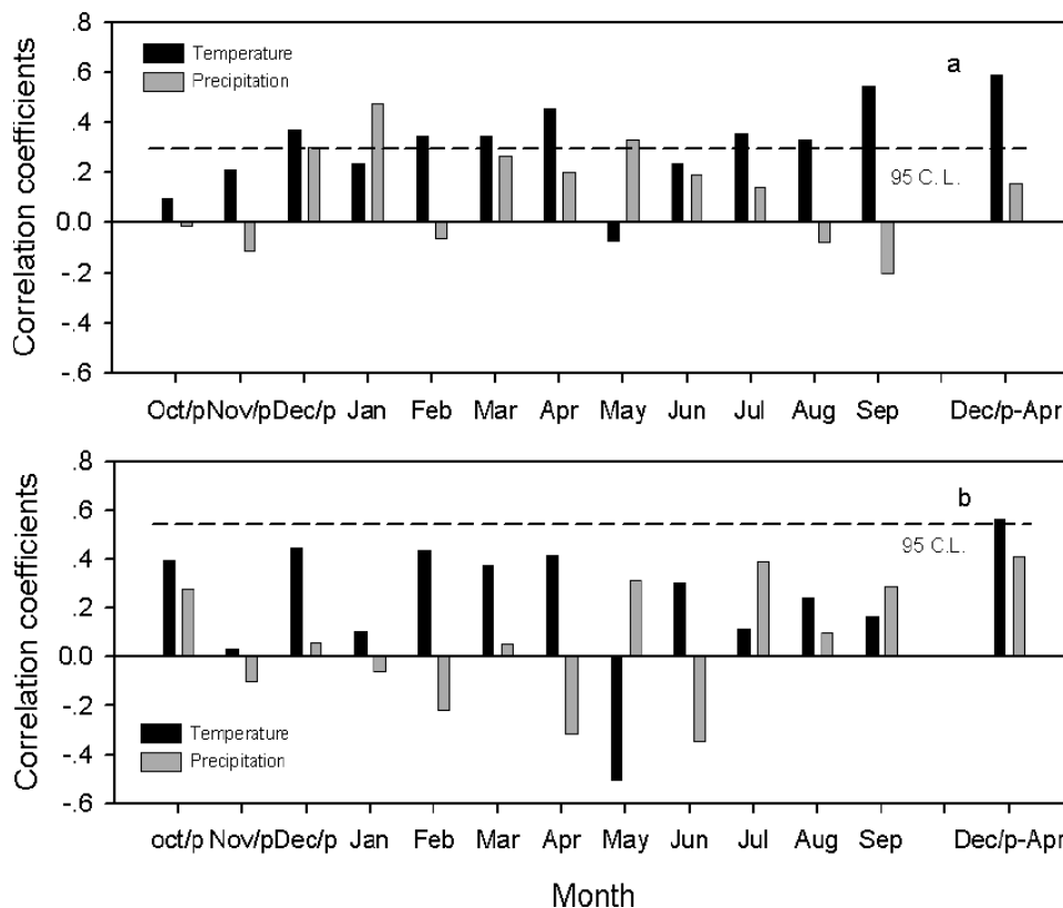
FIGURE 5. Monthly correlation coefficients of tree-ring width chronology and stable carbon isotope series to combined instrumental data from Zhangye and Minle meteorological station from 1958 to 2000. (a) Correlation coefficients for ring width (1 yr) to climate data. (b) Correlation coefficients for stable carbon isotope (3 yr) to climate data. Dashed lines show the 95% confidence limits. p: the climate data of previous growth year.
