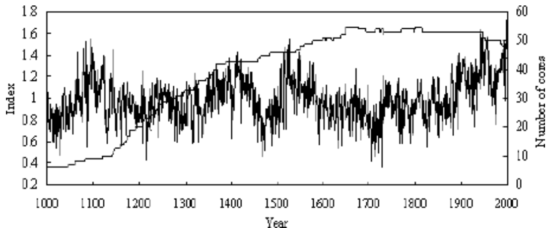
FIGURE 2. Ring-width chronology developed for Qilian juniper in middle Qilian Mountains, along with the sample depth plot.
