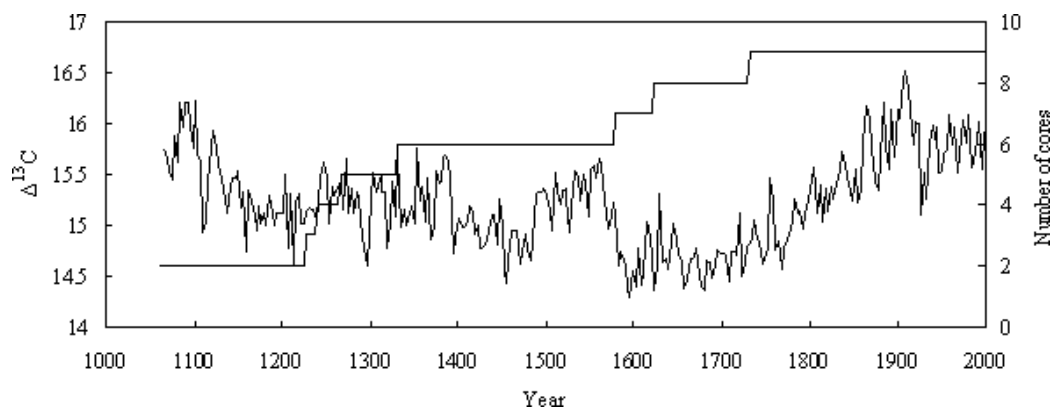
FIGURE 4. Carbon isotope discrimination ( \Delta^{13}\text{C} ) series using equation (1) to eliminate the effects of declining atmospheric \delta^{13}\text{CO}_2 , along with the number of tree cores used for isotope analysis (right axis).
