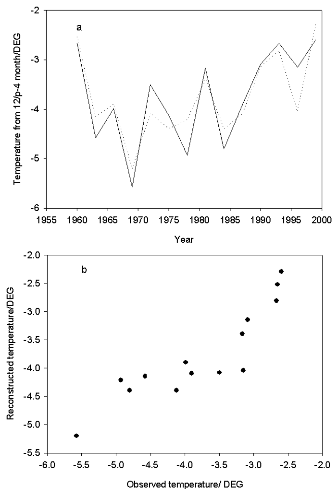
FIGURE 6. Comparison of observed and reconstructed temperature from previous December (12p) to current April (4). (a) Time series plot. Solid line indicates observed value and dash line indicates reconstructed value. (b) Scatter plot.
