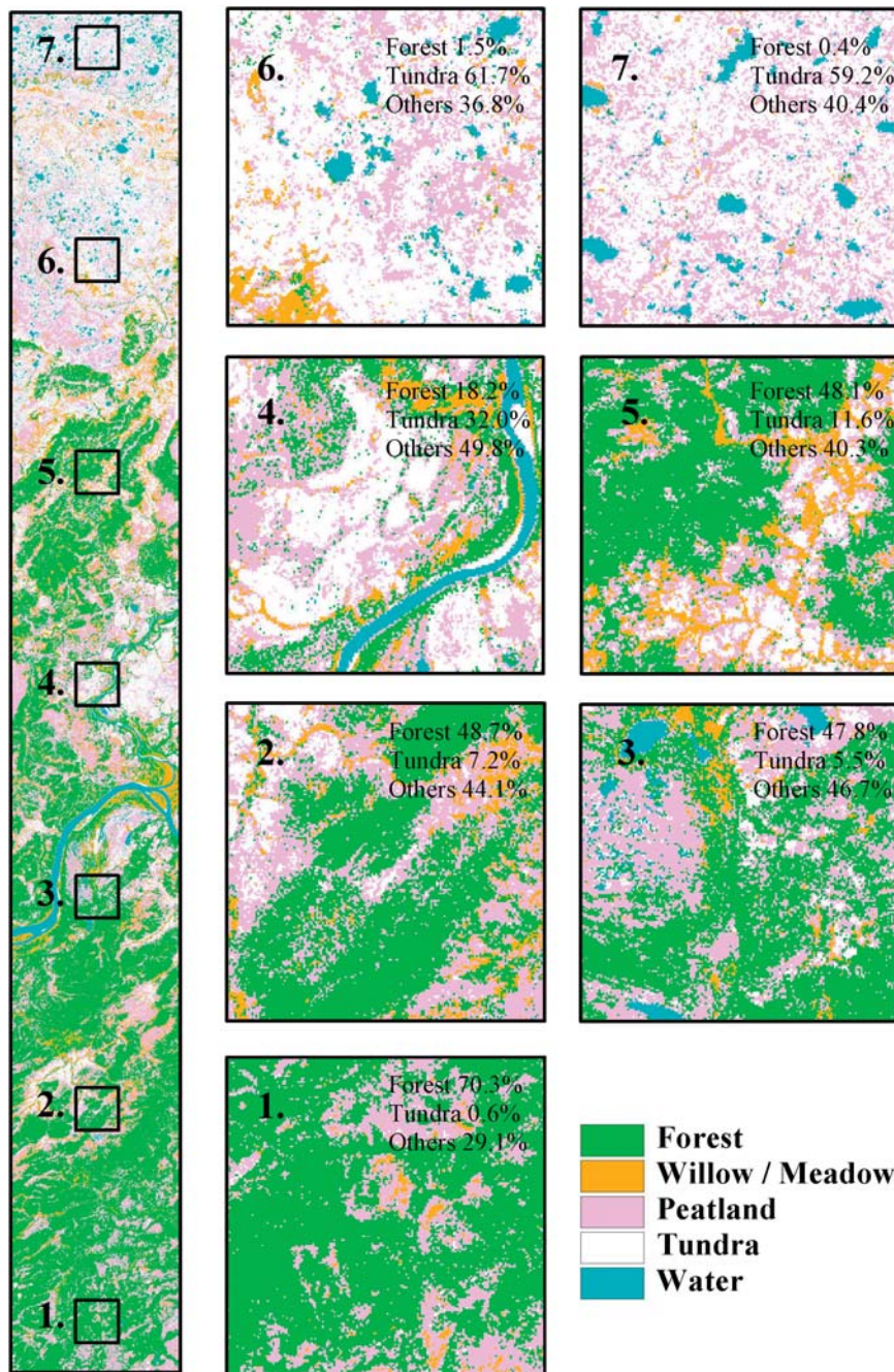
FIGURE 3. The main vegetation types in the satellite image classification illustrating the mosaic nature of the forest-tundra transition zone. On the left is a 25-km-wide and 160-km-long transect from the central Usa basin (see location in Fig 2e). On the right seven more detailed (5 km × 5 km in size) views of the landscape (pixel size 30 m × 30 m, views by 20 km intervals from south to north). The location of the areas is indicated in the figure on the left. The southwest corner of the southernmost view is at 66°00'N, 59°15'E.
