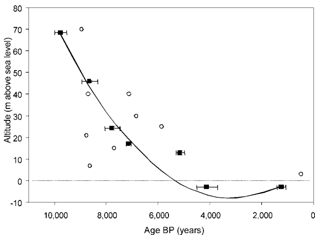
FIGURE 2. Mean sea-level changes in the Mudderbugt region during Holocene. The polynomial fit ( 2 \times 10^{-6} x^2 - 0.0112x + 9.7639 , R^2 = 0.99 ) used in the present study represents dated sediment (solid squares) from eight isolated basins on Arveprinsen Ejland (Long et al., 1999) while open dots represent dated shells and other organic matter from the region (Rasch, 1997). Locations are shown with filled circles in Figure 1.
