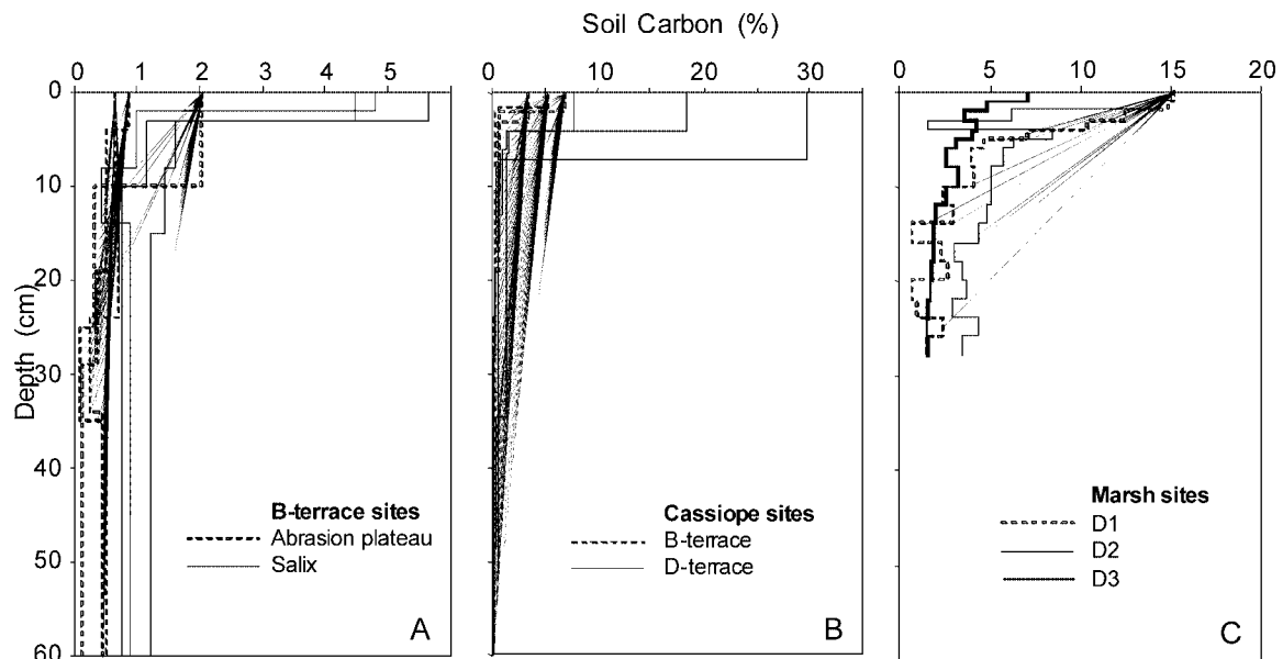
FIGURE 3. Concentration profiles of SOC at A: contrasting vegetation types on terrace B, and B: Cassiope heath sites at two different terraces and C: marsh sites representing a gradient from D1 to D3.
