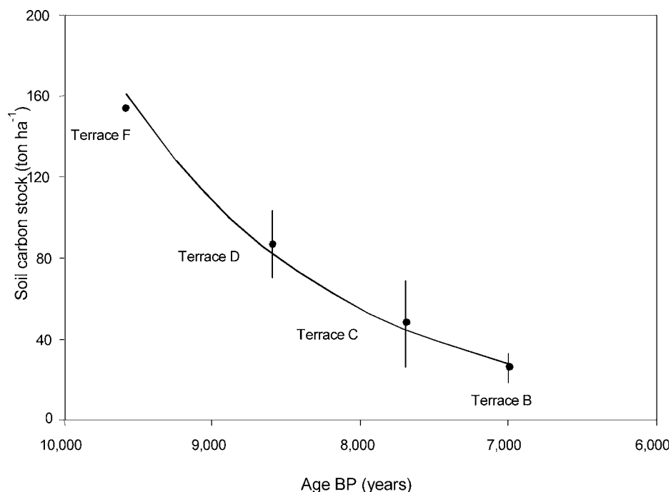
FIGURE 4. Total stocks of SOC to a depth of 60 cm at various terraces. Terrace E has not been sampled and results from terrace A have not been included due to the findings of coal pieces probably imported from nearby coastal coal outcrops. An exponential fit is shown ( 0.0244e^{0.0007x} ; R^2 = 0.9913 ).
