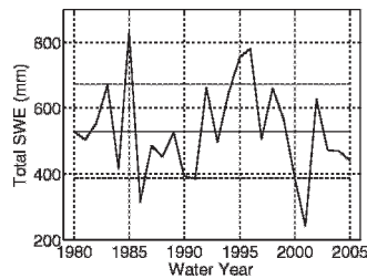
FIGURE 8. Total snow water equivalent (SWE) for each water year (1 October–30 September) measured at Bear Lake SNOTEL site. Horizontal lines are the mean (solid line; 529 mm) \pm one standard deviation (dashed lines; 143 mm).
