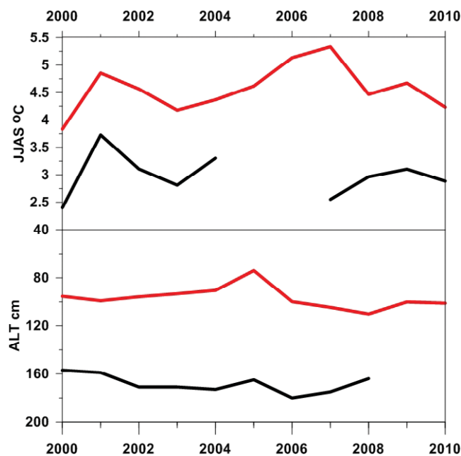
FIGURE 12. Thawing season June, July, August, and September (JJAS) mean air temperatures (upper part) from Airport (red) and Janssonhaugen (black), and the active layer thickness (lower part) as measured in the UNISCALM grid as an average of all the 121 grid points (red) and in the Janssonhaugen borehole (black).
