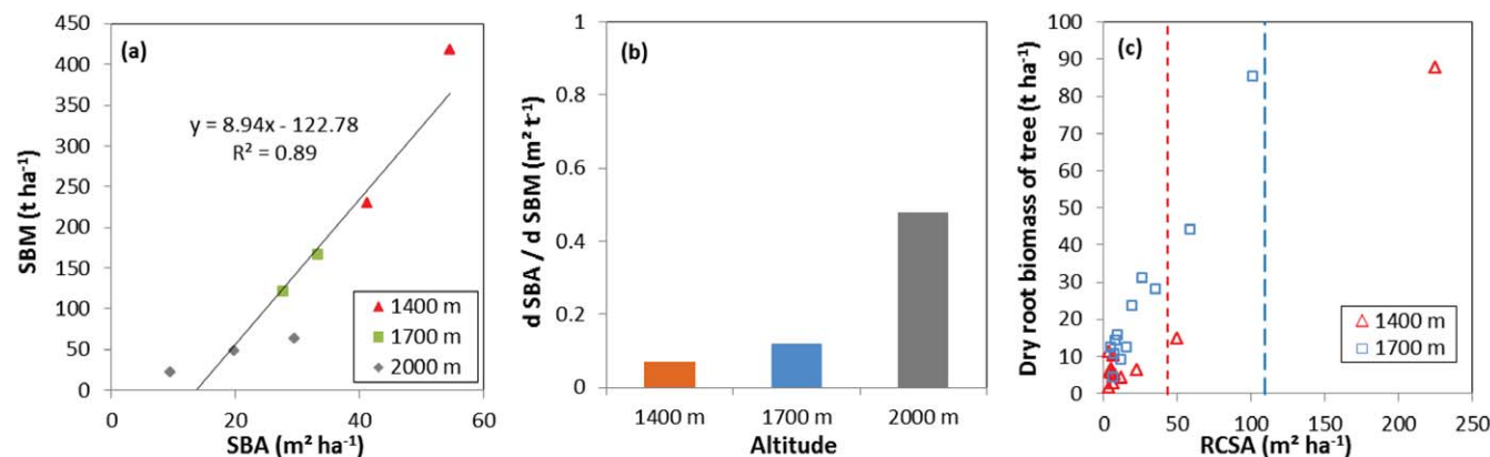
FIGURE 6. (a) Allometric equations estimated stem biomass (SBM, in t\ ha^{-1} ) against stem basal area (SBA, in m^2\ ha^{-1} ); (b) the changed SBA once SBM changes 1 t; (c) measured dry root biomass of tree species against measured root cross sectional area (RCSA, in m^2\ ha^{-1} ) of all diameters, based on the mini-monolith database. In (a), each point represents a sample plot of an altitude; in (c) each point represents an estimated indicator of a monolith (0.3 m in soil depth). The short and long dashed lines in (c) denote the maximum RCSA found in used soil profiles for this present study at 1400 m and 1700 m, respectively.
