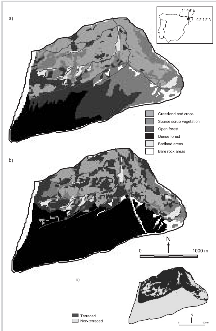
FIGURE 2, A AND B Land-use maps of Cal Rodo catchment in (A) 1957 and (B) 1996. (C) Situation of terraced areas within the catchment.
