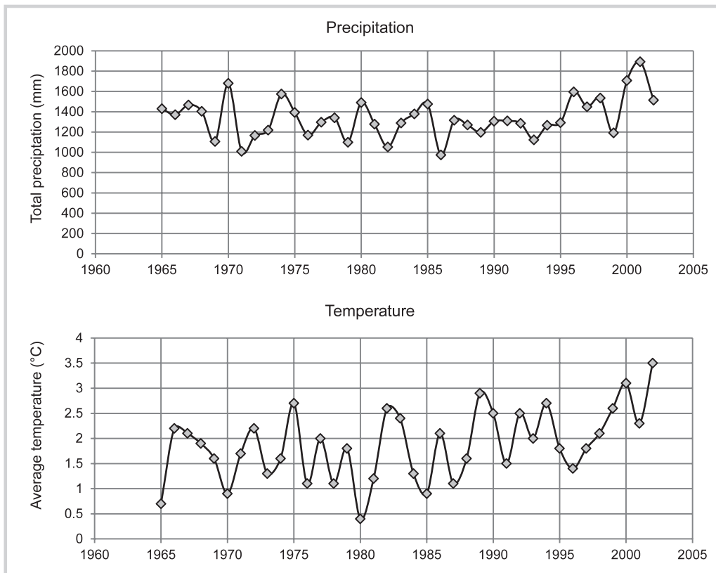
FIGURE 5 Trends in annual average temperature (in degrees Celsius) and annual total precipitation (in millimeters) from 1965 to 2002 at the meteorological station of Skalnaté pleso (1751 masl), Slovak Institute of Hydrometeorology.
