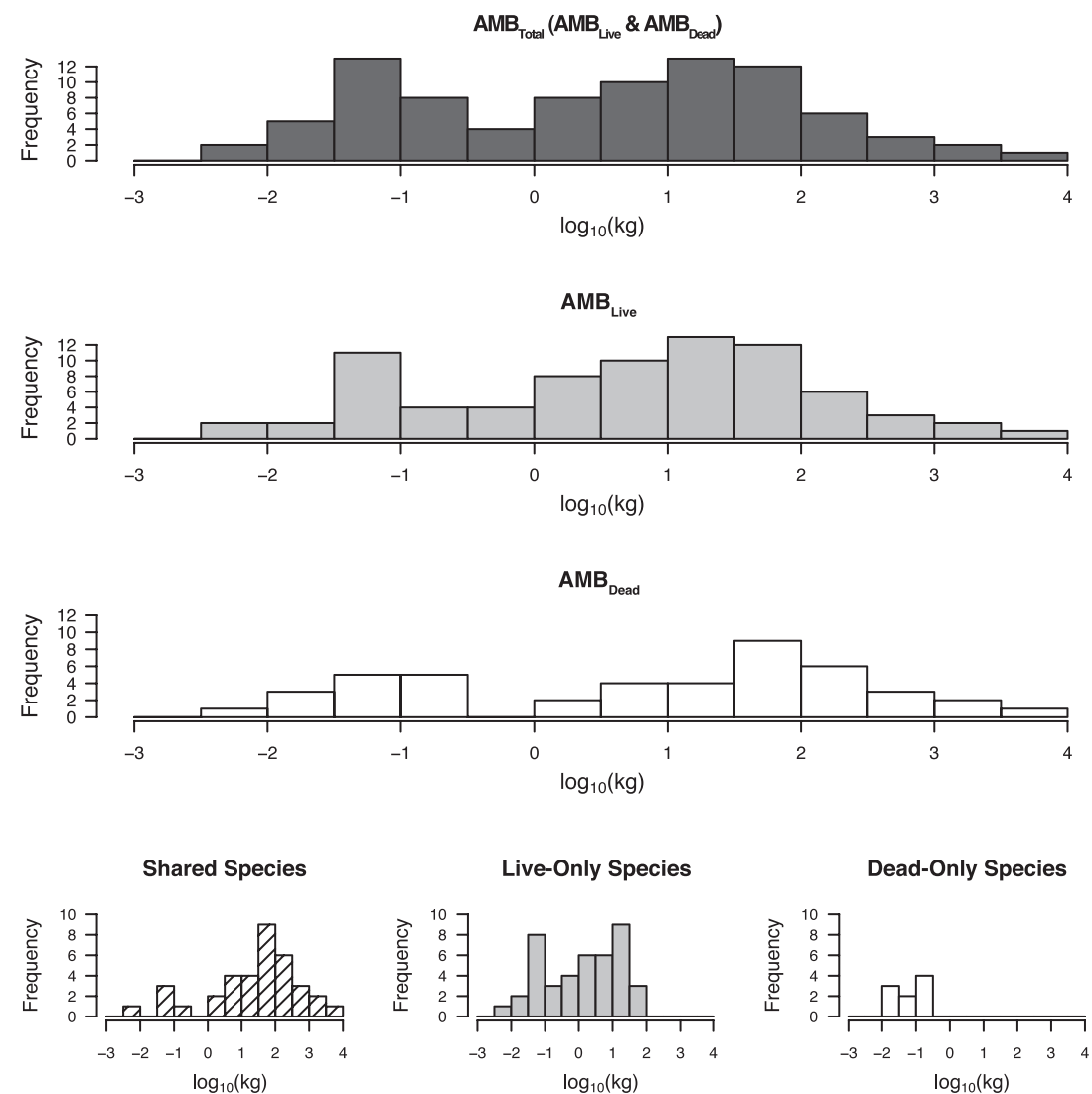
FIGURE 2. Log-transformed body-size (kg) frequency distributions of non-volant mammal species found in Amboseli National Park. AMB Total combines all unique species recovered from sampling the live (AMB Live ) and dead (AMB Dead ) and represents the best estimate for richness and body-size distribution of the whole time-averaged source community. “Shared Species” displays species recovered by both AMB Live and AMB Dead . The body-size frequency distribution of species only found in the live (“Live-Only Species”) and dead (“Dead-Only Species”) are also provided. Complete listing of species in Supplementary Appendix A.
