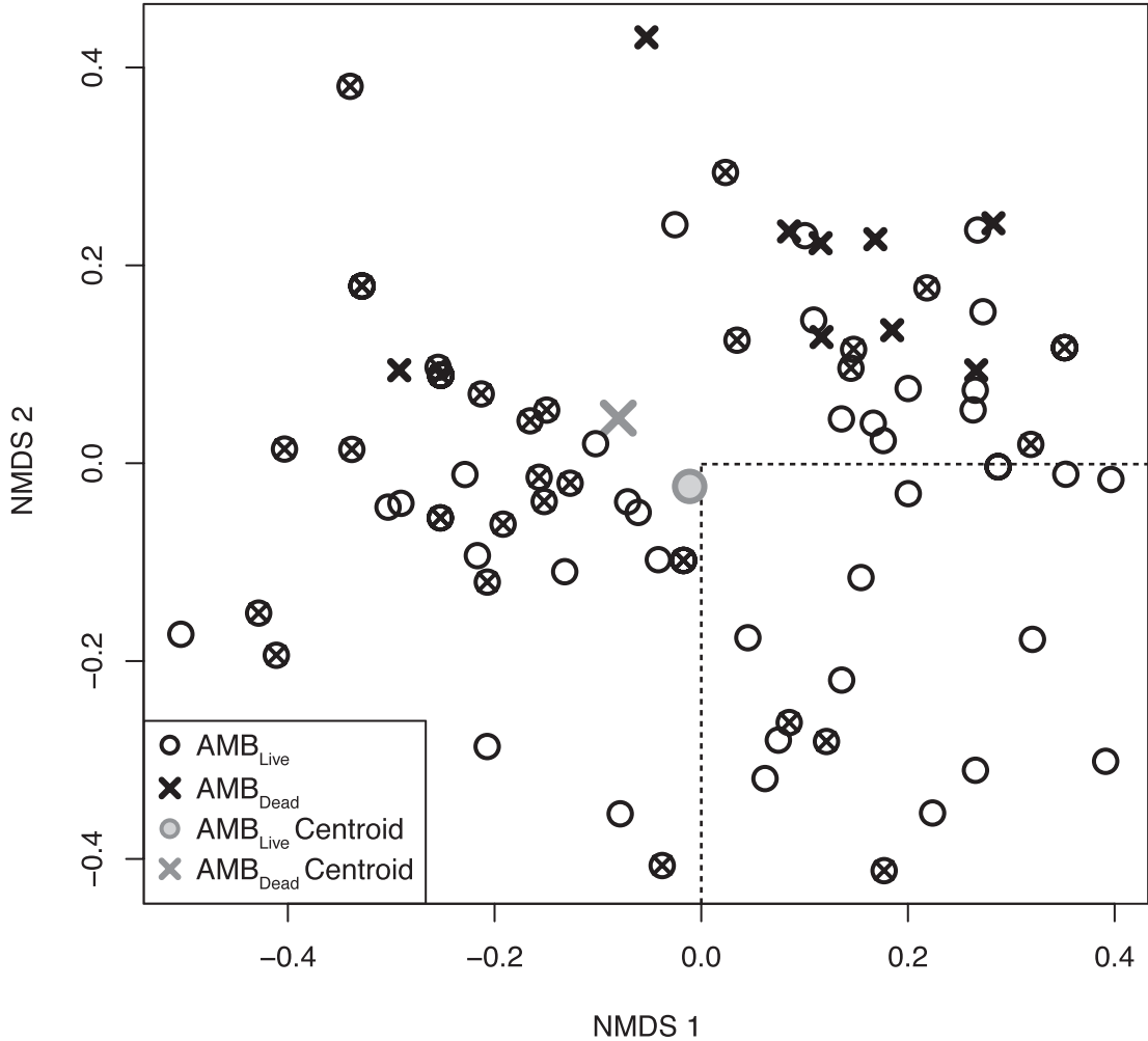
FIGURE 7. Nonmetric multidimensional scaling of four ecological traits for the total Amboseli mammal community (AMB Total ; Stress = 0.125). Species recorded by AMB Death are small X's. Species documented in AMB Live are open circles. Though not demarcated, the global (AMB Total ) centroid is located at [0, 0]. A gap in coverage by AMB Death in the lower-right quadrant (dashed box) corresponds to ecospace constructed by species that (1) consume other animals (invertebrates, meat, bone), (2) shelter in underground cavities, and (3) are active during many periods of the day (Supplementary Fig. S2).
