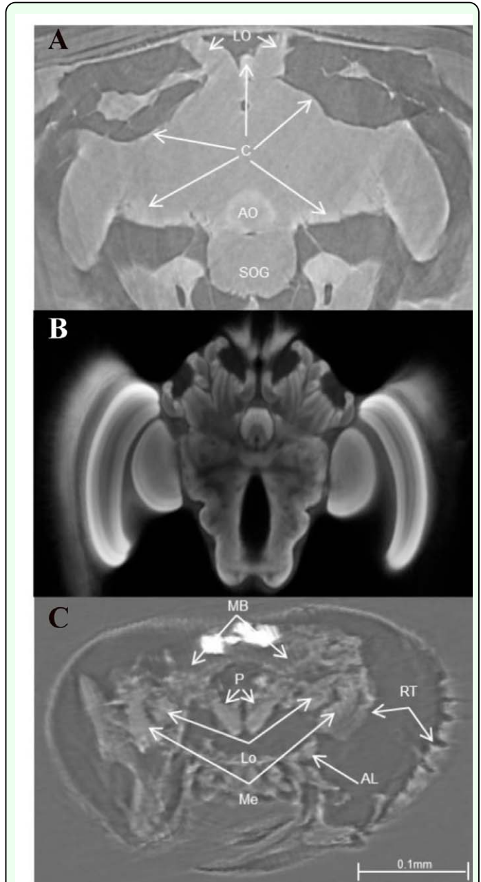
Figure 4. (a) A 2D axial view of a live honey bee brain showing perfusion of contrast medium (C) into peripheral regions. Arrows indicate areas of higher concentration. At 30 minutes post bolus injection into the haemolymph, the lateral ocelli (LO) and aorta (AO) contained more contrast than the sub oesophageal ganglion (SOG). (b) A comparative 2D axial view from the bee brain atlas ( http://www.neurobiologie.fu-berlin.de/beebrain/Default.html ) that was reconstructed from imaging data from two-channel confocal microscopy scans. (c) An axial view of the head capsule of an ancient stingless bee Proplebeia abdita (Greco et al. 2011) trapped in amber. The brain of this 20 million years old bee was particularly well preserved, as evidenced by the optic lobes including the medullae (Me) and lobulae (Lo), antennal lobes (AL), protocerebral lobes (P), and the mushroom bodies (MB). The retinal zone (RT) was also well preserved. High quality figures are available online.
