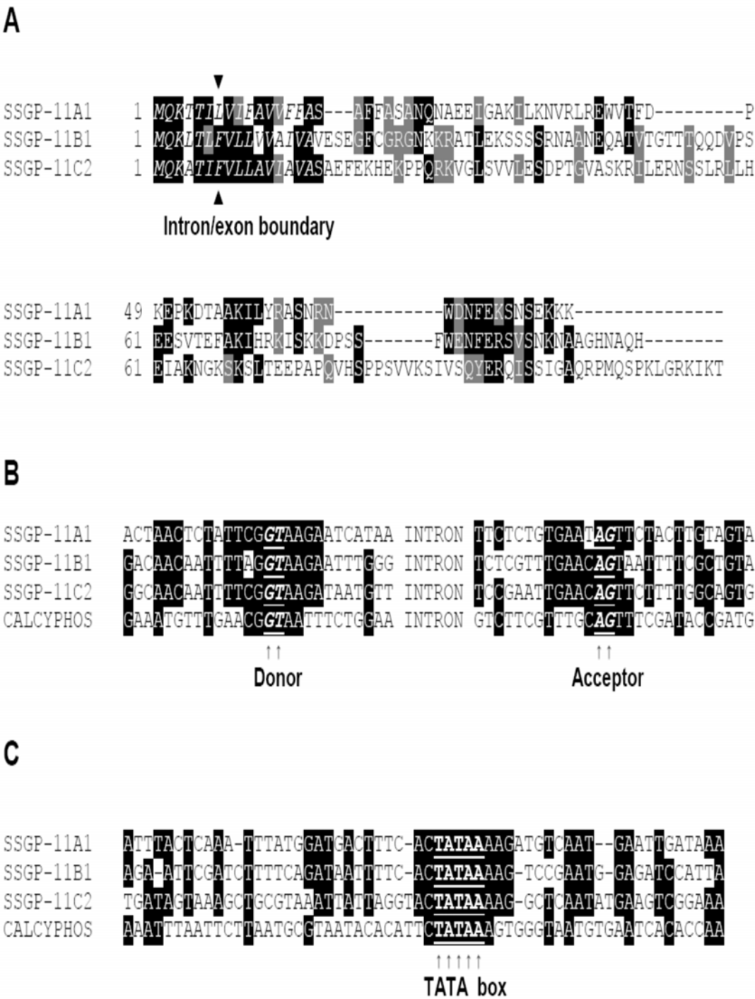
Figure 4. Structural similarity among the SSGP-11A1, SSGP-11B1, and SSGP-11C2-encoding genes. A: Amino acid sequence alignment. The first 16 amino acids (italic) constitute a putative secretion signal peptide. Black residues indicate identical amino acids between at least two proteins. Gray residues represent conserved substitutions. White residues represent amino acid differences. Dashed lines indicate absence of amino acids in specific proteins. The conserved location of the intron (between F and V) is indicated by the symbols ▲ and ▼. B: Conservation in nucleotide sequence at intron/exon splicing boundaries. The alignment was made using standard program (see Experimental Protocol section). CALCYPHO represents calcyphosine, an unrelated gene from the Hessian fly. Black areas represent residues identical at least 3 sequences. Intron splicing donor and acceptor are bold and underlined and indicated by arrows. C: Conservation in the promoter region. Putative “TATA” box is bold and underlined and indicated by arrows.
