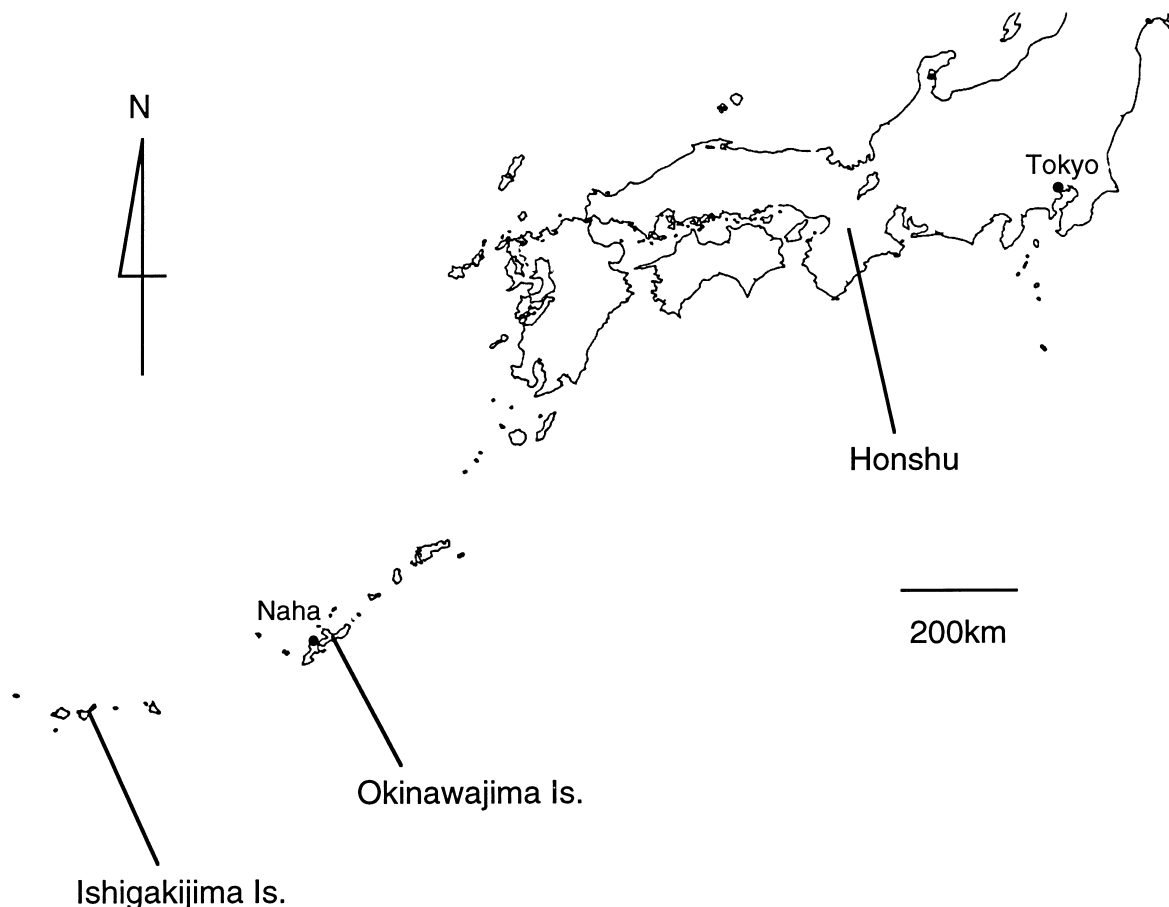
Fig. 1. A map of the Ryukyu Islands and neighboring mainlands of Japan.
