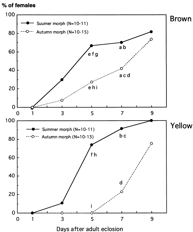
Fig. 6. Comparison of ovarian maturation between brown- and yellow-type females. P > 0.05 (Fisher's exact probability test), non-significant between the common letters on the same days. The p -values were adjusted by a sequential Bonferroni procedure (Rice, 1989).
