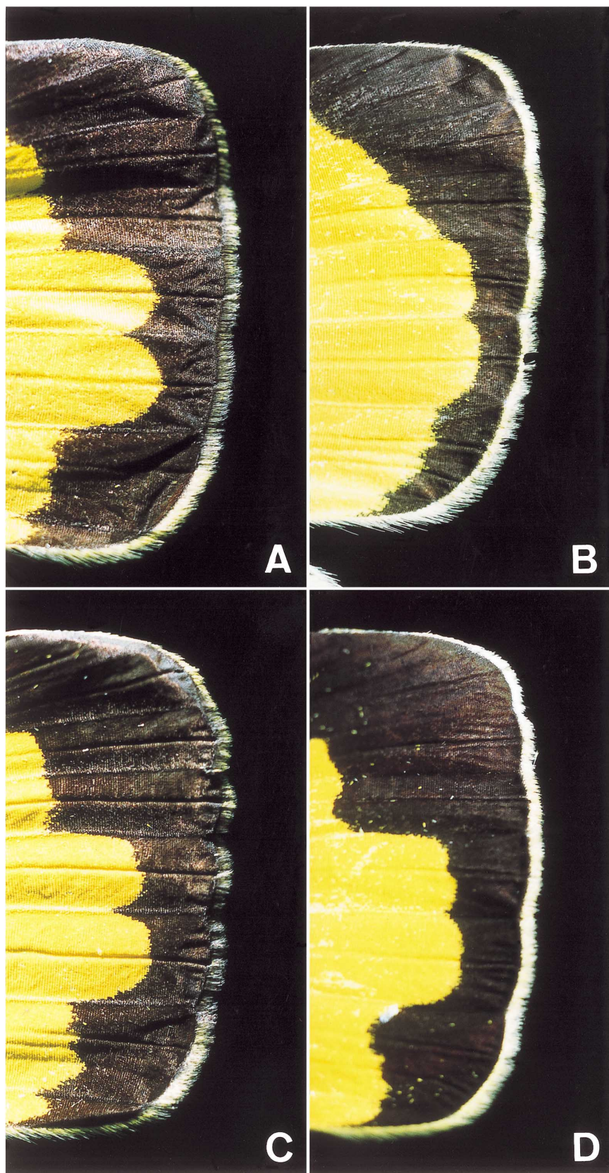
Fig. 2. Fringe coloration of forewing upperside in E. hecabe (L) from Okimawa-jima Is. and neighboring regions. Brown (A) and yellow (B) type individuals from Okinawa-jima Is. Brown type from Ishigaki-jima Is. (C) and yellow type individuals from Honshu (D).
