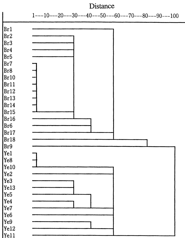
Fig. 4. Clustering of wild-caught females (brown and yellow types) based on median values of B- and M-scores of the first generation at 20°C and 12L–12D.
