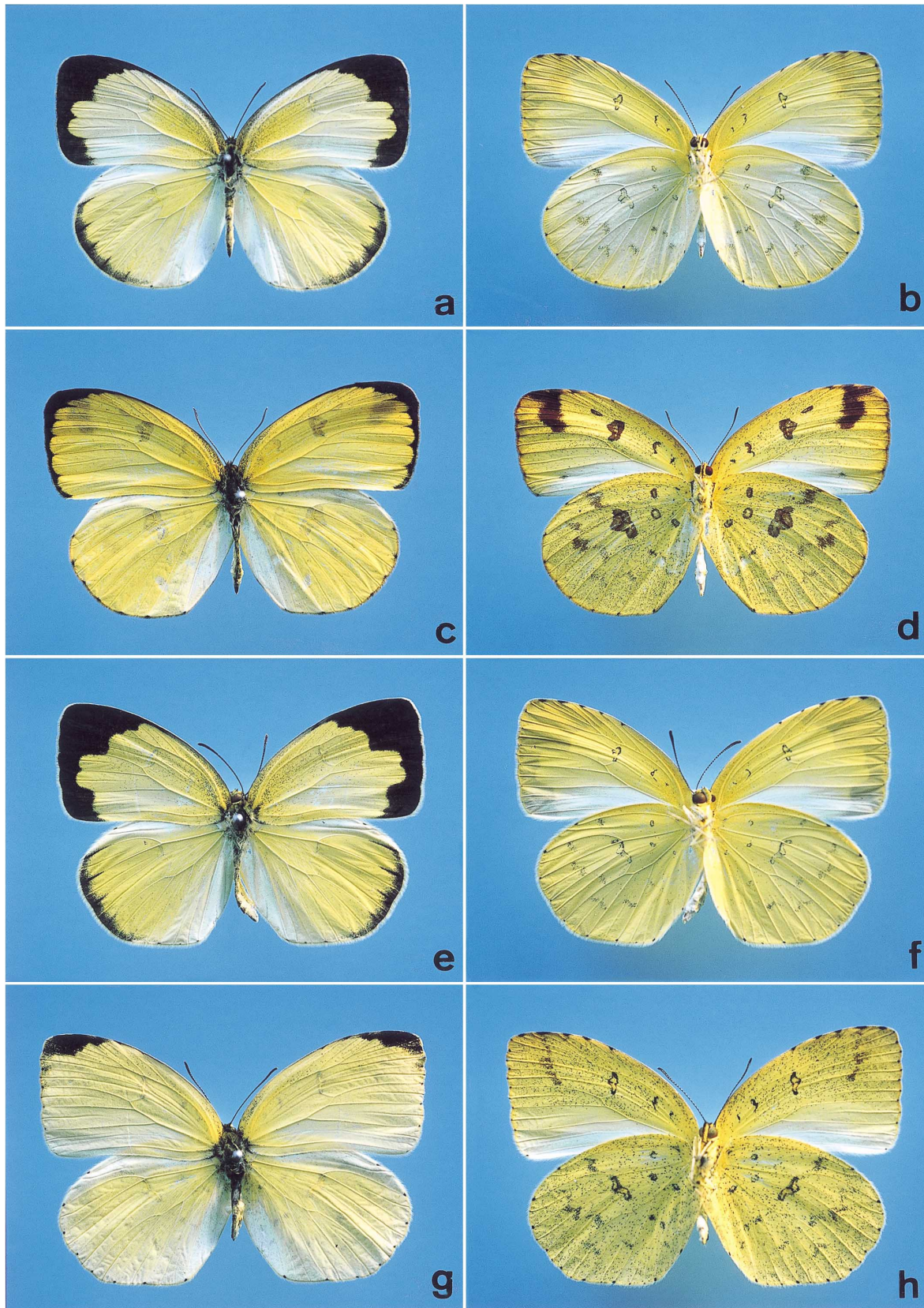
Fig. 3. Summer and autumn morphs of the adults in Eurema hecabe (L.) from Okinawa-jima Is..(a–d) Brown type. (e–g) Yellow type. (a) Upperside (B0 for B-score) and (b) underside (M0 for M-score) of typical summer morphs. (c) Upperside (B4) and (d) underside (M3) of typical autumn morphs. (e) Upperside (B0 for B-score) and (f) Underside (M0 for M-score) of typical summer morphs. (g) Upperside (B6) and (d) Underside (M1) of typical autumn morphs. Here the female specimens are shown.
