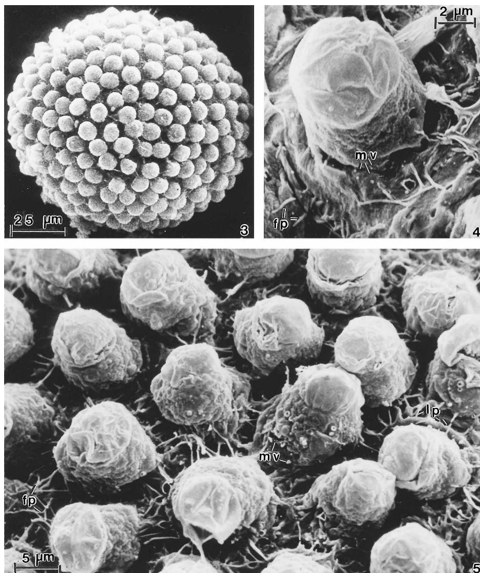
Figs. 3–5. SEM micrographs of S. plicata eggs: general view (Fig. 3); details of fc (Fig. 4) and of the fc layer (Fig. 5). fp =filopodia; lp =lamellipodia; mv =microvilli.
