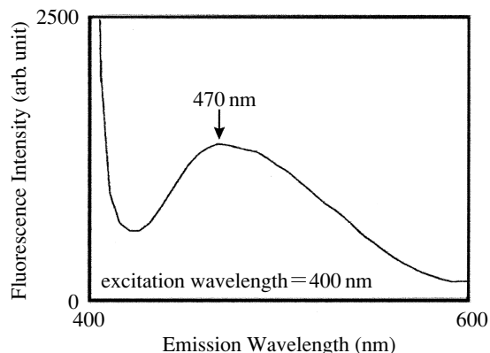
Fig. 5. Emission spectrum obtained from the contour peak shown in Fig. 3. The excitation wavelength was 400 nm.
