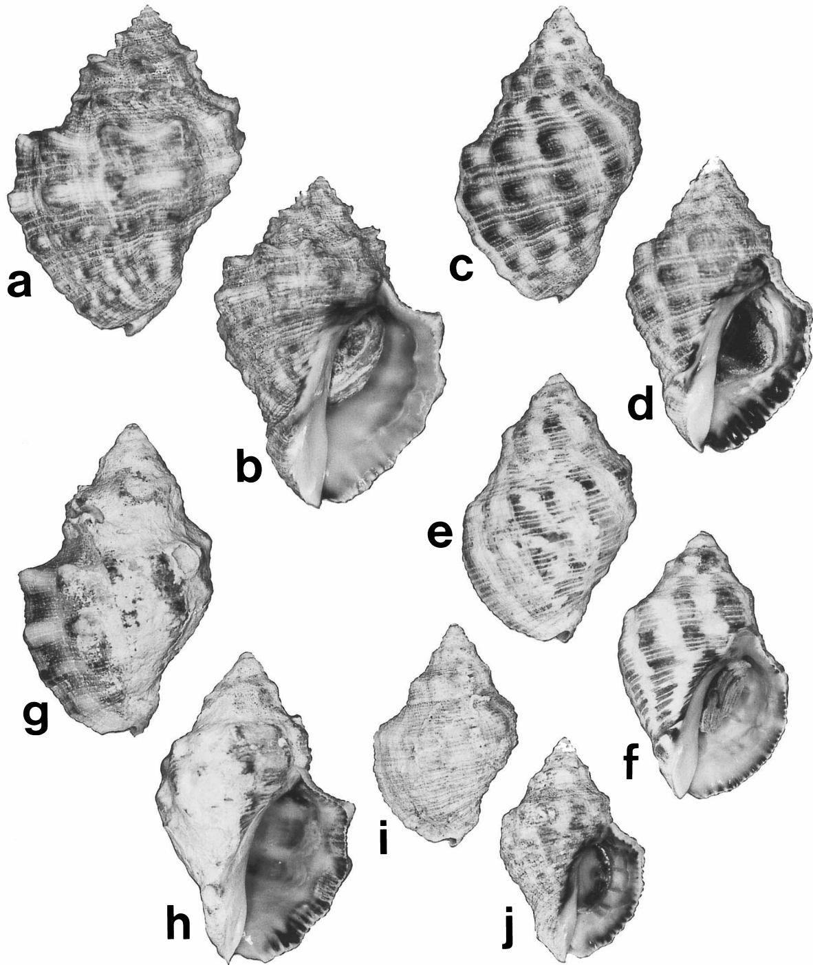
Fig. 2. Shells of Thais species. (a, b) Thais bitubercularis (Lamarck), Chiku, Taiwan, SH=36.7 mm; (c, d) Thais clavigera (Küster), Ta-an (24 21'N, 120 34'E), Taiwan, SH=33.2 mm; (e, f) Thais jubillaea Tan and Sigurdsson, Kuantan, Malaysia, SH=29.9 mm; (g, h) Thais luteostoma (Holten), Cape d'Aguilar, Hong Kong, SH=34.9 mm; (i, j) Thais rufotincta Tan and Sigurdsson, Tungkang, Taiwan, SH=25.2 mm.
