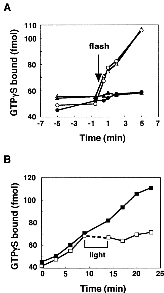
Fig. 4. Time course of GTP \gamma S-binding to the octopus retinal G-protein G q in the presence of rhodopsin and t-rhodopsin. A: GTP \gamma S bound to the G q upon illumination of rhodopsin (open circles) or t-rhodopsin (open triangles). Basal GTP \gamma S-binding without illumination was not observed either in the presence of rhodopsin (closed circles) or t-rhodopsin (closed triangles). B: GTP \gamma S bound to the G q in the presence of t-Acid Metarhodopsin in the dark (closed squares). GTP \gamma S binding to the G q was inhibited when t-Acid Metarhodopsin was illuminated with orange light (for 5 min from 9 to 14 min) to form rhodopsin (open squares).
