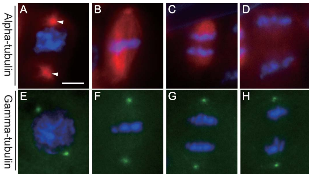
Fig. 3. Embryos of parthenogenetic D. pulex during cleavage division (mitosis), with spindles (pink, top row) indicated by immunofluorescence visualization of \alpha -tubulin and centrosomes (green, bottom row) by visualization of \gamma -tubulin. Chromosomes are counter-stained with DAPI (blue). The spindle is spindle-shaped and astral; \gamma -tubulin is present only at the spindle poles. (A, E) Prophase; arrowheads in (A) indicate asters. (B, F) Metaphase. (C, G) Anaphase. (D, H) Telophase. Scale bar = 5 \mu m.
