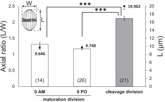
Fig. 4. Spindle axial ratio ( L/W ; see spindle diagram at upper left) and spindle length for abortive meiosis and cleavage division in parthenogenetic D. pulex ( ***P < 0.001 , t -test). The large bars represent mean values for the axial ratio (left axis), with range lines indicating the standard deviation. Numbers in parentheses below the large bars indicate the sample size. Small circles with range bars represent mean axial length (right axis) and the standard deviation.
