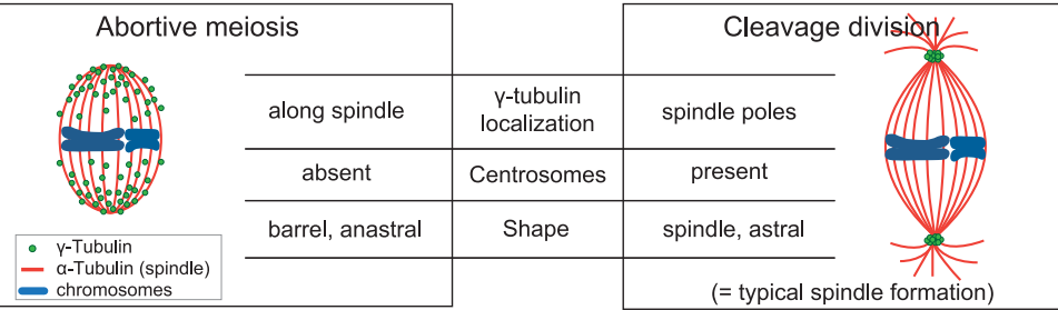
Fig. 5. Schematic diagram comparing spindle morphology between abortive meiosis and cleavage division in parthenogenetic D. pulex .
