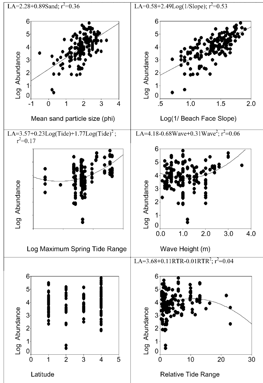
Figure 4. Scatter plots of relationships between log(total abundance per transect) and six physical parameters. Where significant, regression lines are shown.
