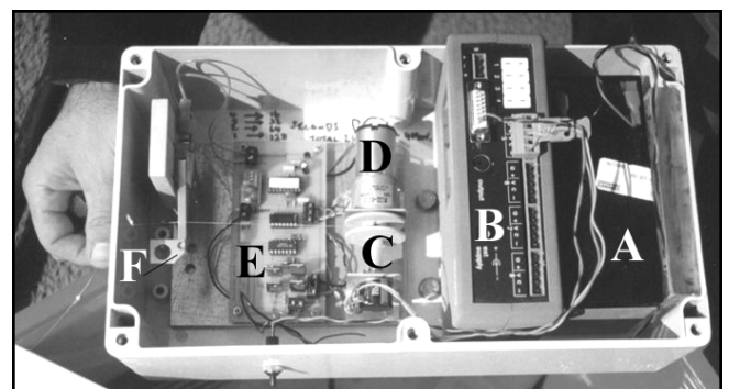
Figure 3. Interior of the electronic control box. A – 12v battery, 7 Ah; B – Data logger; C – pulley wheel for cord; D – motor; E – control circuitry; F – Tension sensor micro-switch which detects slack in the cord upon contact with the sea bed.
