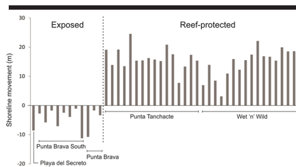
Figure 6. Immediate shoreline response driven by Hurricane Wilma.
