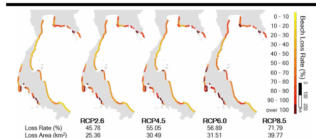
Figure 5. The projected beach loss rate and area in 2081–2100 relative to 1986–2005 based on ensemble mean sea level rise for 4 RCP scenarios.
