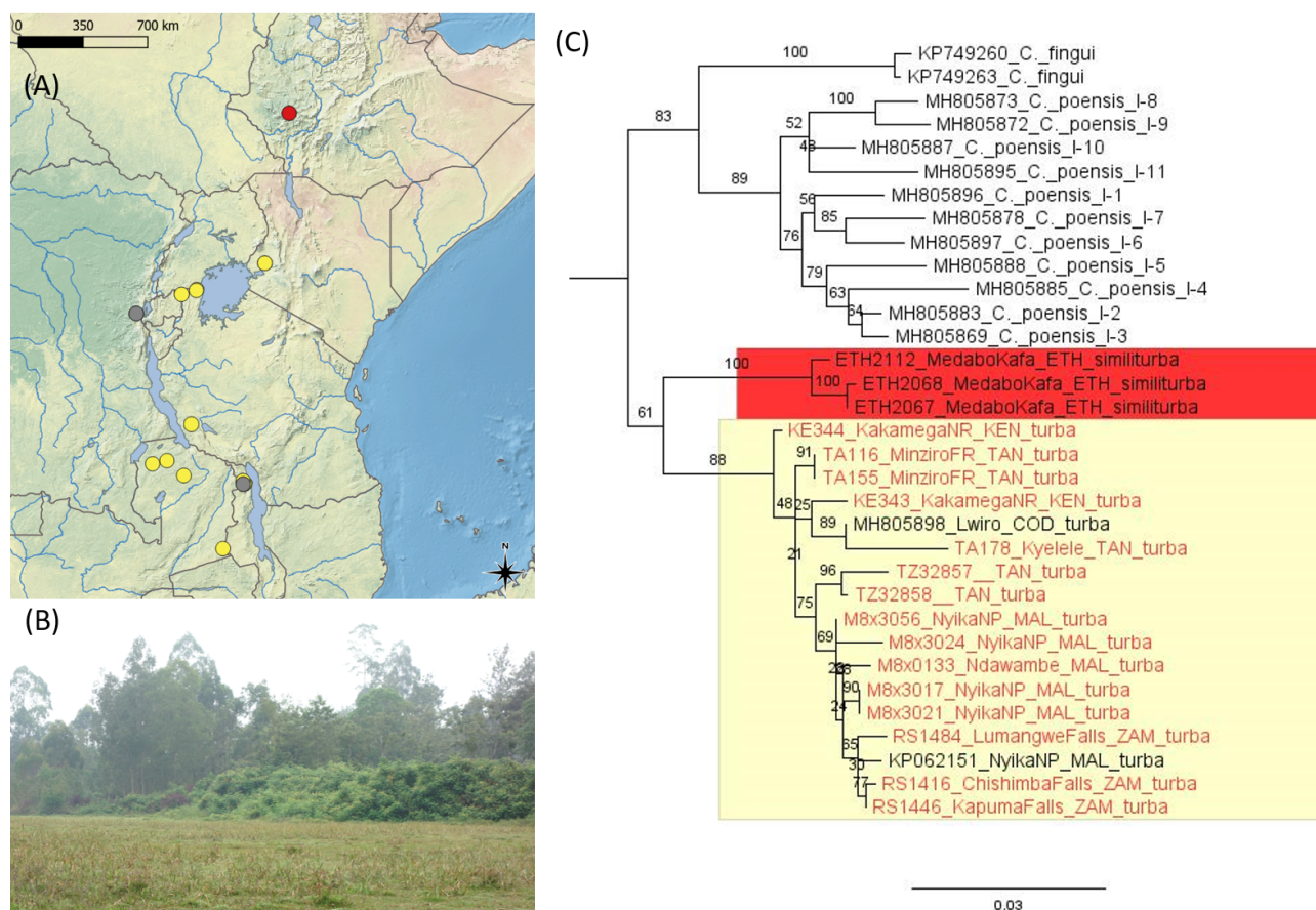
Fig. 2. (A) Distribution of Crocidura similitorba sp. nov. (red point) and Crocidura turba (yellow points – new localities of specimens genetically confirmed in this study; grey points – localities previously reported by Nicolas et al. 2019). (B) Habitat of C. similitorba sp. nov., close to Medabo village (Kafa zone, south-western Ethiopia). Currently this represents the only known locality of the species. (C) Phylogenetic tree of the Central and East African part of the Crocidura poensis species complex (sensu Nicolas et al. 2019) estimated by maximum likelihood analysis of cytb sequences. Sequences of C. similitorba sp. nov. are highlighted in red, and those of its sister species C. turba in yellow background. New sequences of C. turba are shown in red, GenBank sequences are in black. The West African species of the complex (lineages IV-IX sensu Nicolas et al. 2019) and more distant outgroups are not shown.
