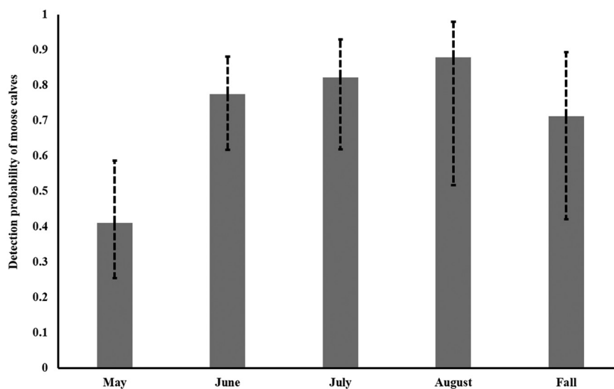
Figure 2. Monthly estimates of moose calf-at-heel detection probabilities (p) from Colorado. Maximum likelihood detection probabilities and 95% confidence intervals, reflected by solid gray bars and dashed black lines, respectively, were estimated using an occupancy modelling framework.
