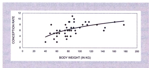
Figure 5. Relationship between the eviscerated body weight of the mother and the conception rate ( y = 3.7457\ln(x) - 10.075 ; r = 0.5648 ; N = 41 ).
