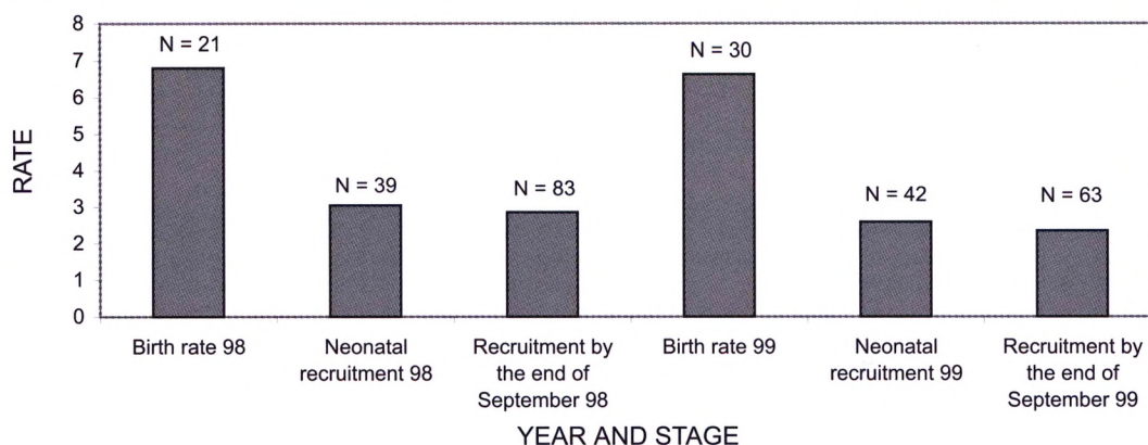
Figure 6. Estimated birth rate and recruitment to the female population during the two years of the investigation.
