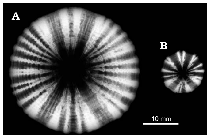
Fig. 9. Radiographs of vertebrae of the mackerel shark Carcharomodus escheri (Agassiz, 1843), MNU 071-20, from Groß Pampau, the middle-late Miocene. A. Precaudal vertebra, same as in Fig. 6Q. B. Caudal abdominal/caudal vertebra, same as in Fig. 7J.
