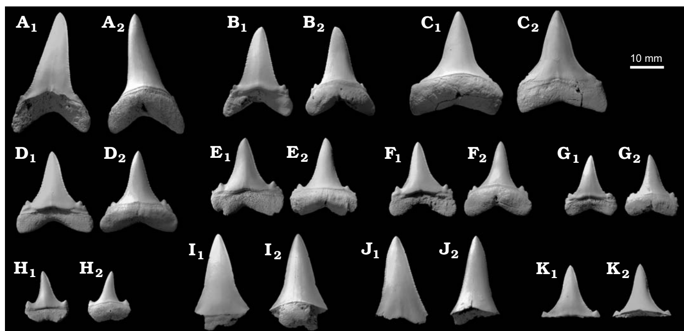
Fig. 11. Lower jaw teeth of the mackerel shark Carcharomodus escheri (Agassiz, 1843), MNU 071-20, from Groß Pampau, the middle-late Miocene. A. Lower left anterior tooth. B. Lower left intermediate tooth. C–H. Lower lateral teeth. Labial ( A_1 – H_1 ) and lingual ( A_2 – H_2 ) views. I. Incomplete anterior lower lateral tooth. J, K. Incompletely mineralized lower replacement teeth.
