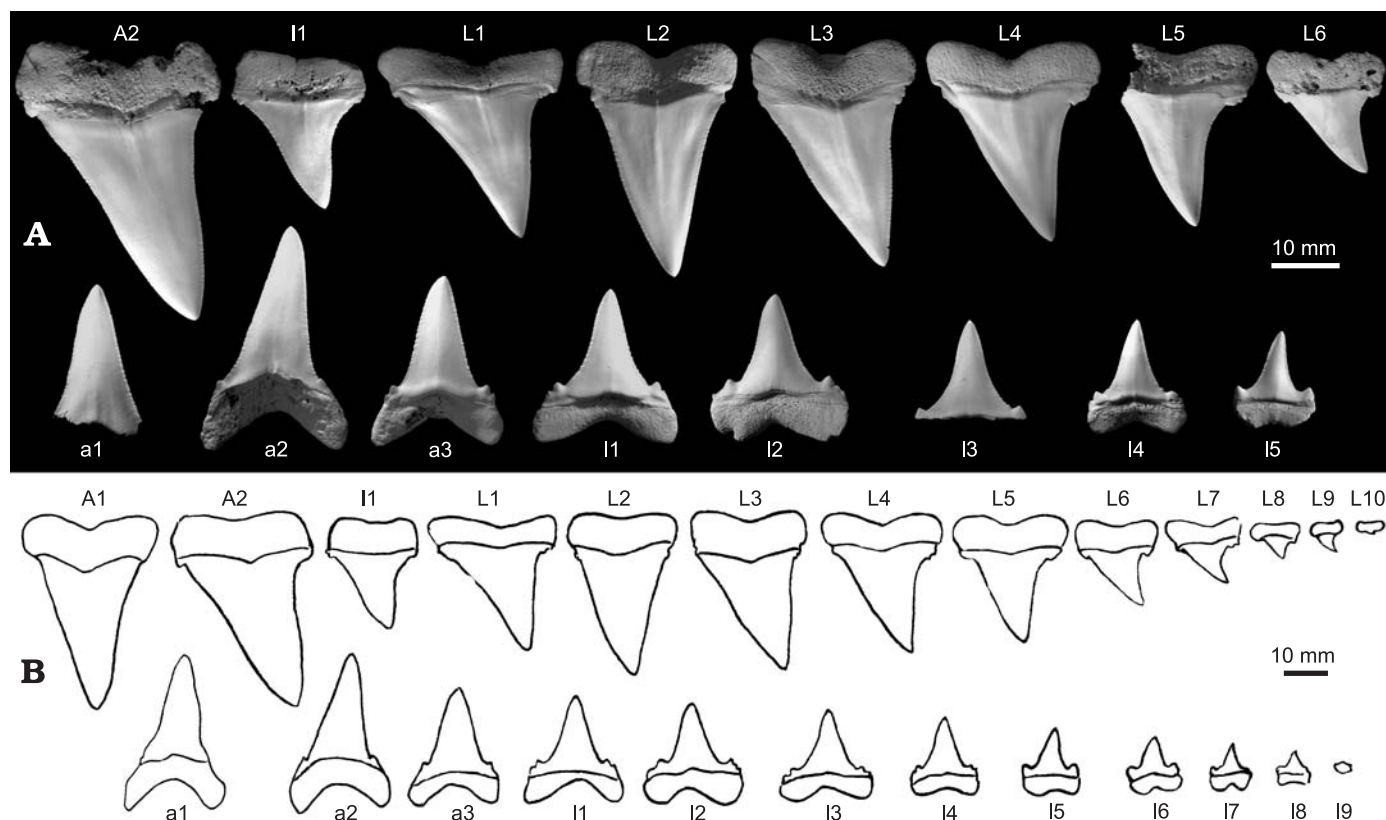
Fig. 12. Reconstructed left upper and lower tooth rows of the mackerel shark Carcharomodus escheri (Agassiz, 1843), in lingual view. A. Reconstruction based on preserved teeth. B. Drawing of the completely reconstructed dentition based on preserved teeth and comparisons with living lamnid sharks.
