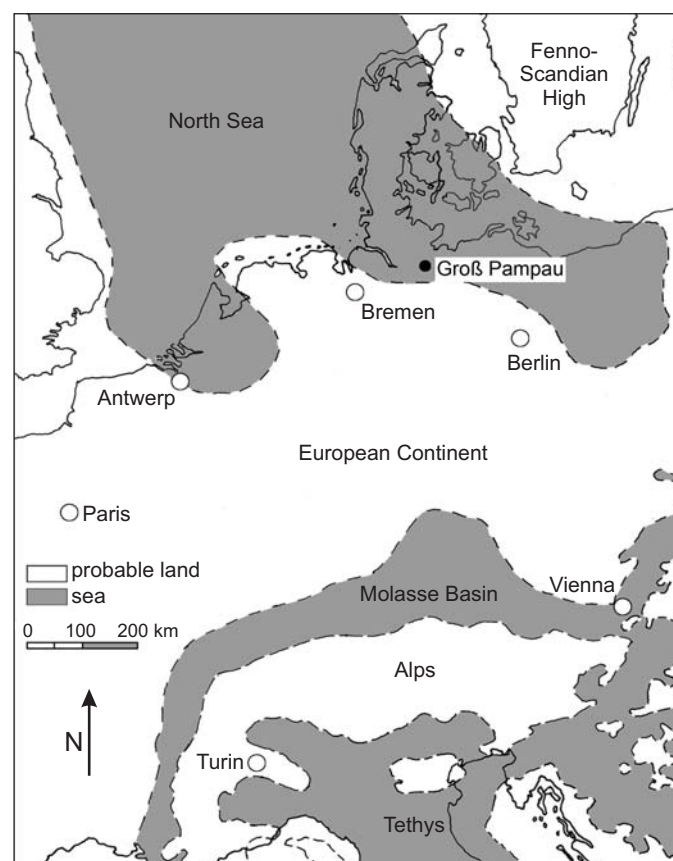
Fig. 1. Palaeogeographic map of mid-west Europe during the middle–late Miocene (compiled from Steininger et al. 1985; Huuse 2002; Rasmussen 2005) showing the locality Groß Pampau in a bay of the North Sea where the partial skeleton was recovered.
