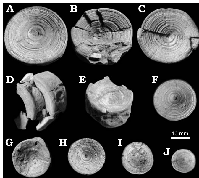
Fig. 7. Posteriormost precaudal and caudal vertebrae of the mackerel shark Carcharomodus escheri (Agassiz, 1843), MNU 071-20, from Groß Pampau, the middle-late Miocene, from anterior (A) to posterior (J).
