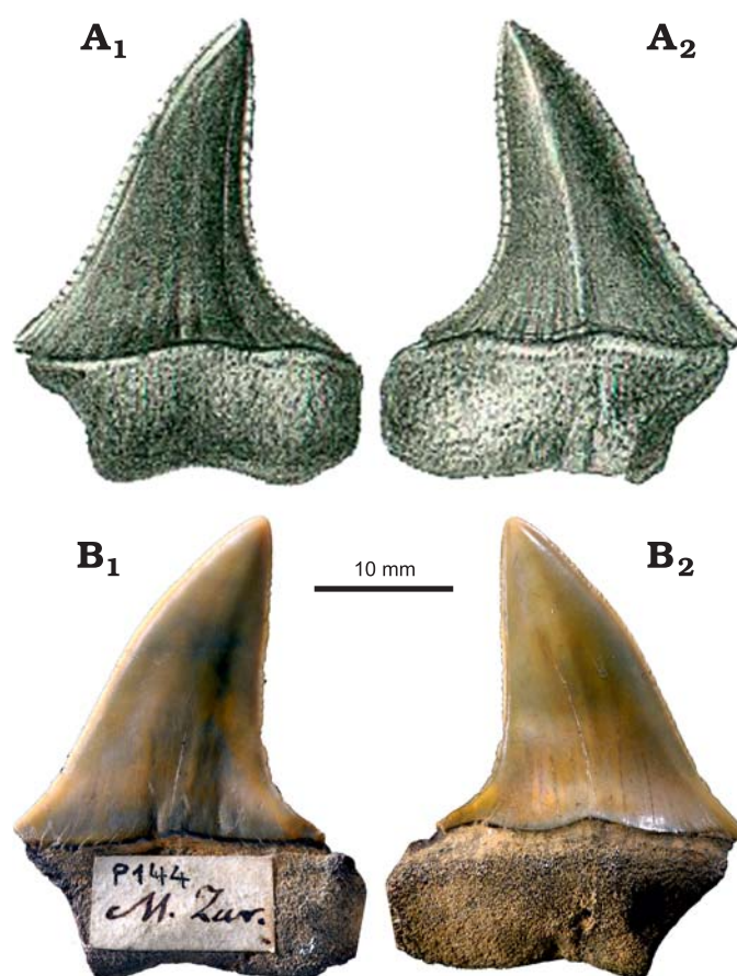
Fig. 4. Holotype of the mackerel shark Carcharomodus escheri (Agassiz, 1843) from the Upper Marine Molasse (Burdigalian–Ottangian, early Miocene) of Switzerland. A. Original drawings of Agassiz (1843: pl. 36: 16–18), in labial (A 1 ) and lingual (A 2 ) views. B. Photographs of holotype (ETZ 0000000001750), in labial (B 1 ) and lingual (B 2 ) views.
