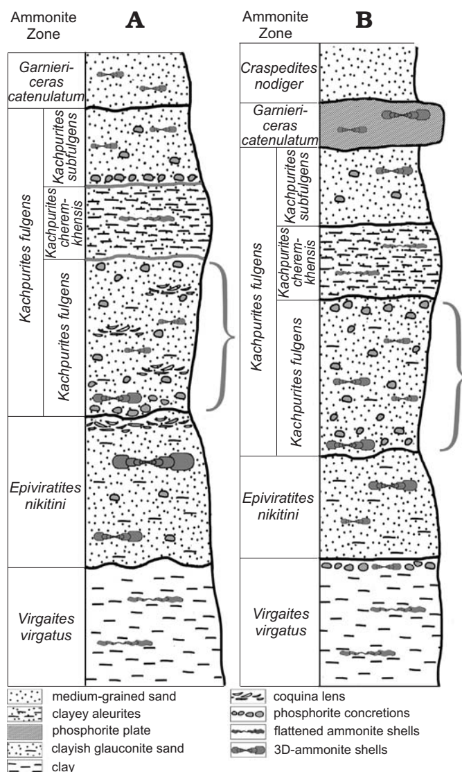
Fig. 2. Stratigraphic column of the localities. A. Mnevniki, Moscow. B. Eganovo, Moscow area. The braces mark the horizon from which the described ammonites have been collected. Ammonite zones (see Rogov and Starodubtseva 2014). The total thickness of the layers is about 2 m.
